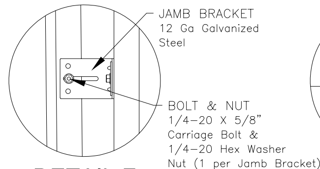
DETAIL F
