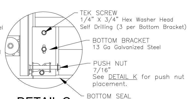
DETAIL C
