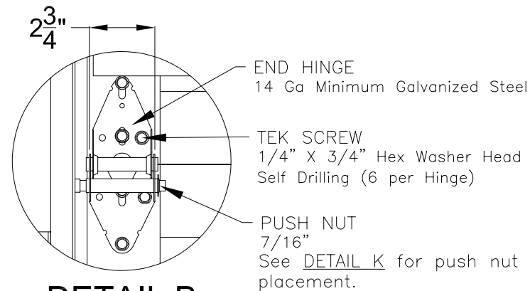
DETAIL B
