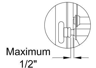
DETAIL K
