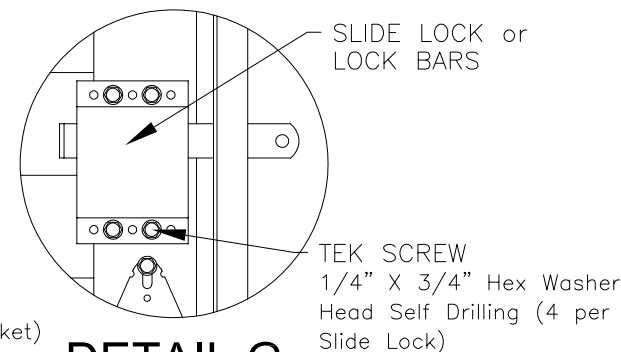
DETAIL G
