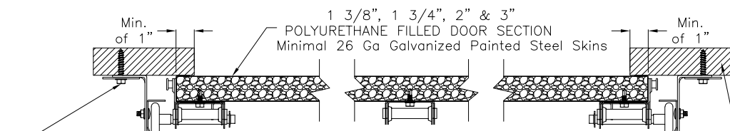
DETAIL H
