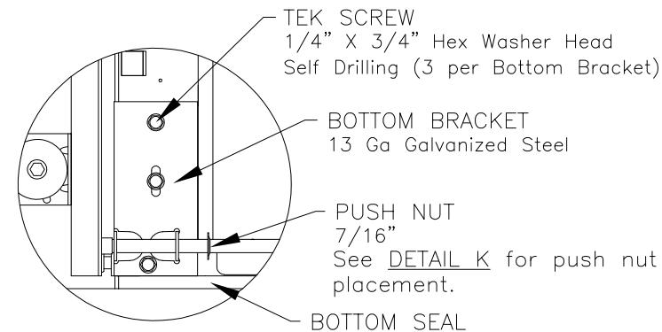
DETAIL C
