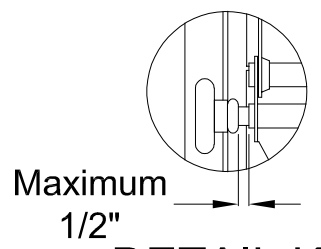
DETAIL K
