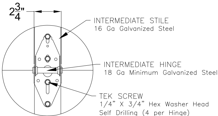
DETAIL D
