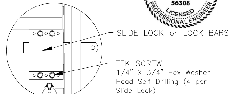
DETAIL G
