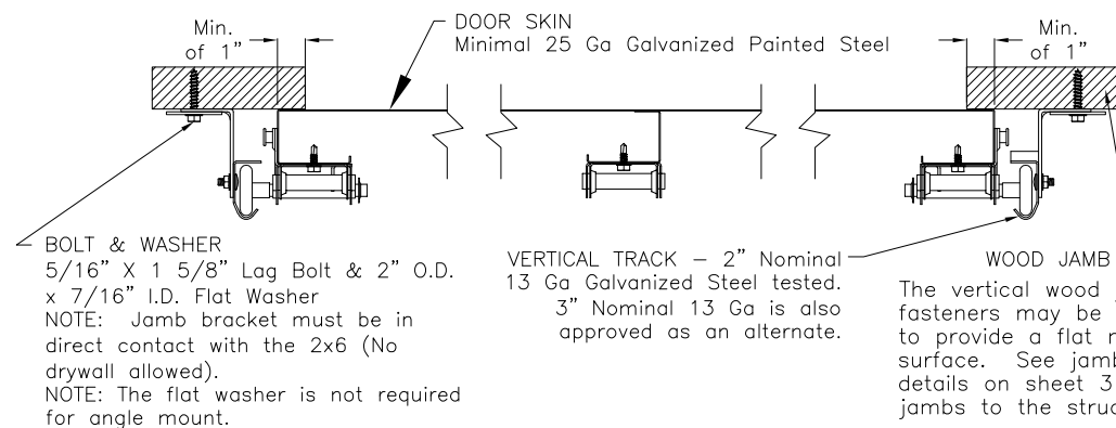
DETAIL H
