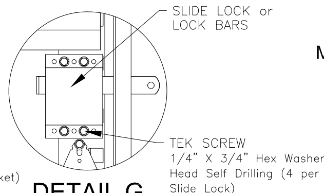
DETAIL G
