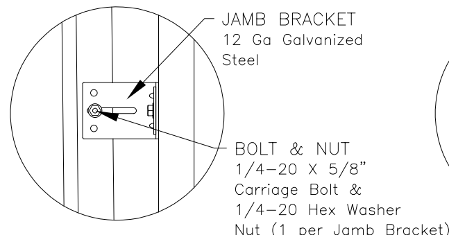
DETAIL F
