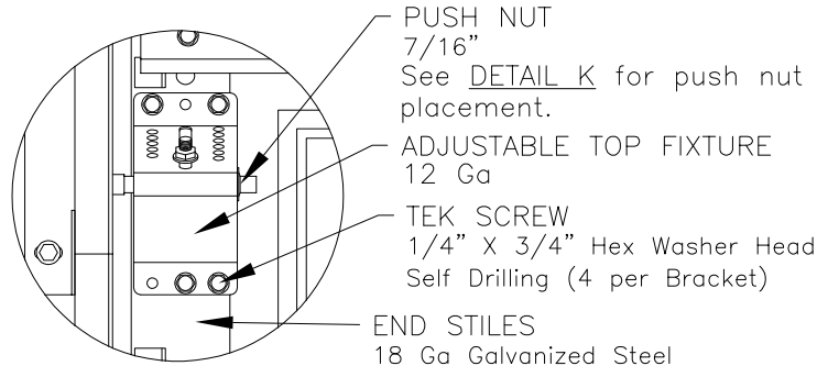
DETAIL A
