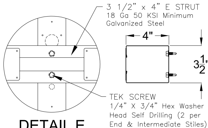
LOW HEADROOM TOP BRACKET
