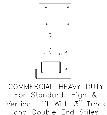
ALTERNATE BOTTOM BRACKETS
