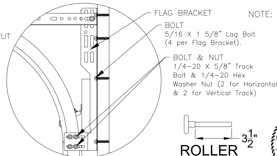
DETAIL F
