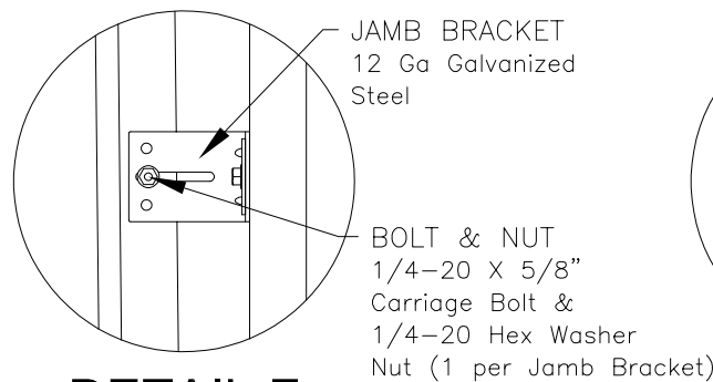
DETAIL F
