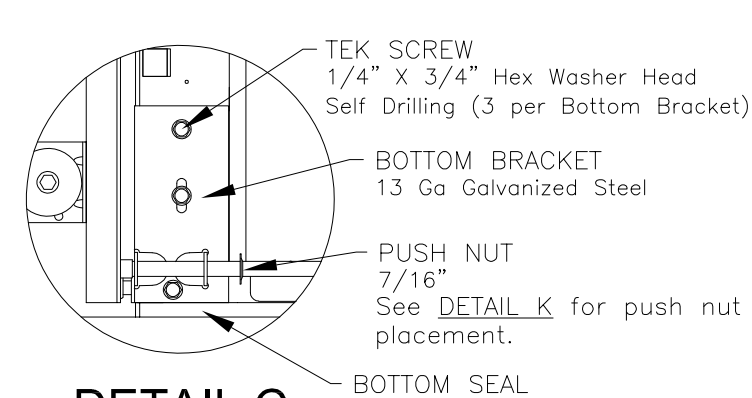
DETAIL C
