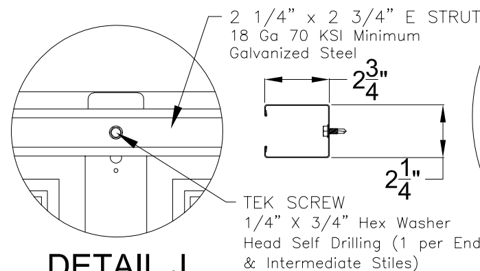
COMMERCIAL For Standard, High & Vertical Lift With 2" Track and Single End Stiles
