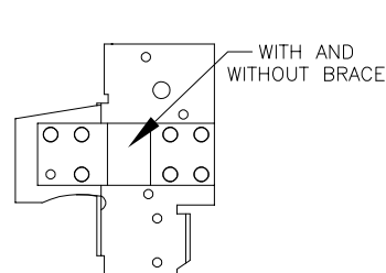
RESIDENTIAL & LIGHT COMMERCIAL For Low Headroom With 2" Track and Single End Stiles
