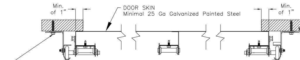
DETAIL H
