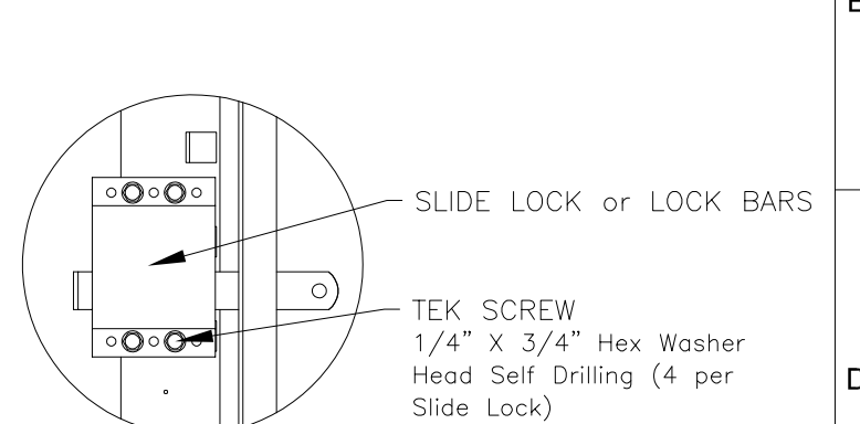
DETAIL G
