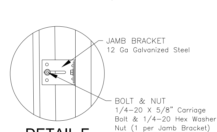
DETAIL F
