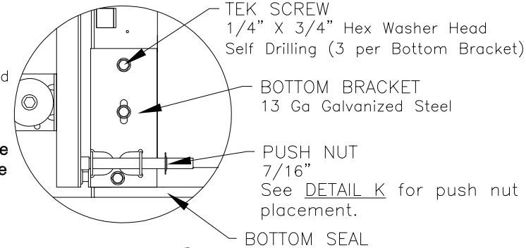
DETAIL C
