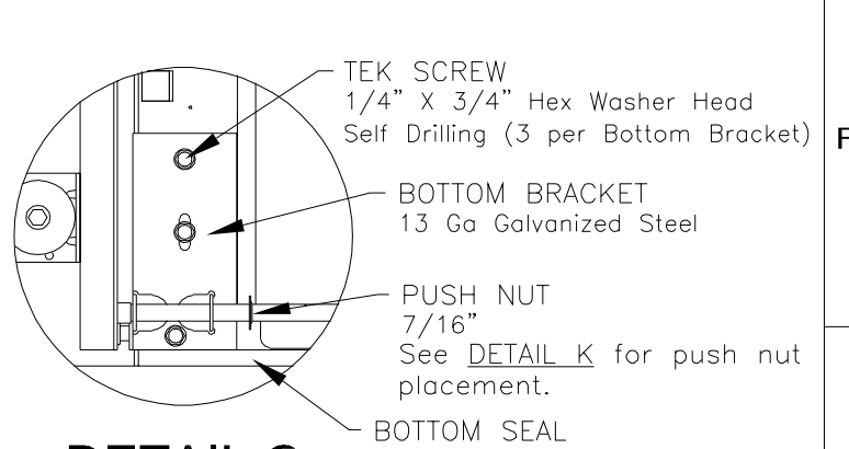
DETAIL C
