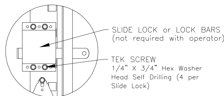
DETAIL G
