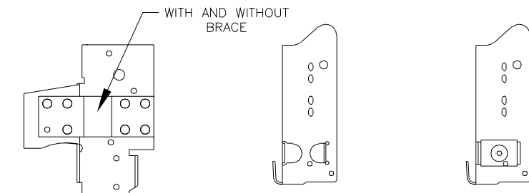
DETAIL D
