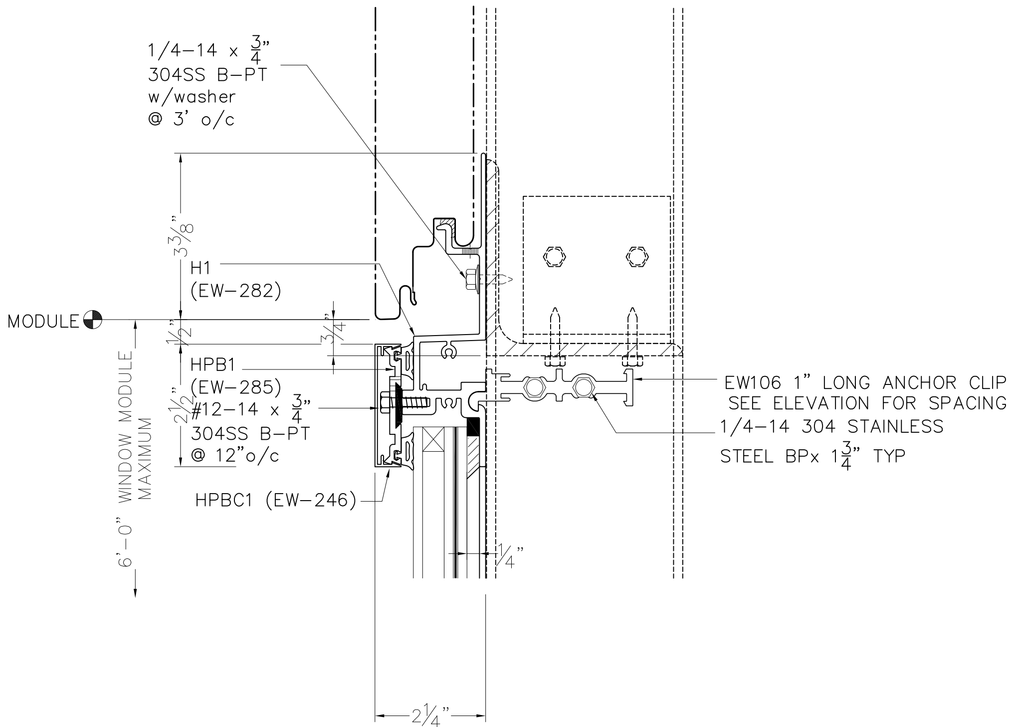
SECTION AA TYPICAL SECTION THRU WINDOW HEAD AT JAMBS AND VERTICAL MULLION SEE GLAZING DETAILS SHEET 11
