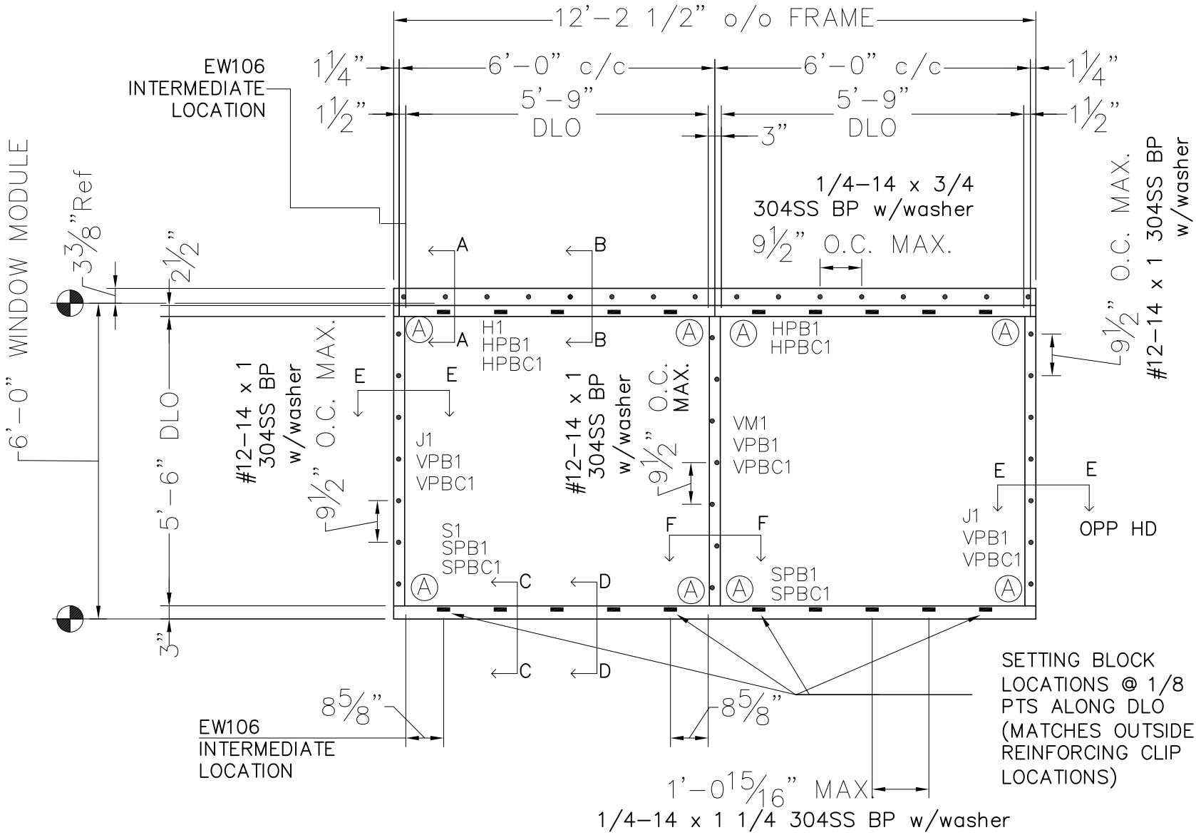
WINDOW FRAMING ELEVATION
