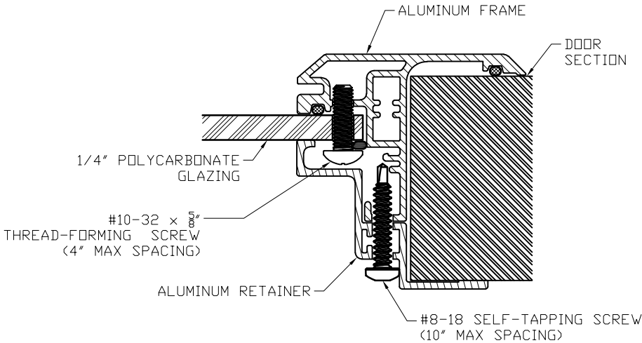
IMPACT-RESISTANT ASSEMBLY DETAILS DRAWING 104432-A
