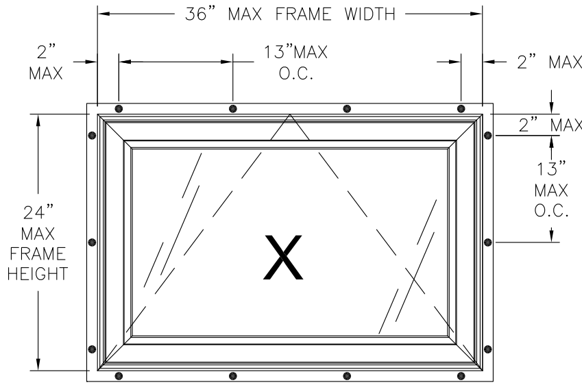
4350 AWNING WINDOW - NON REINFORCED EXTERIOR VIEW FIN INSTALLATION
