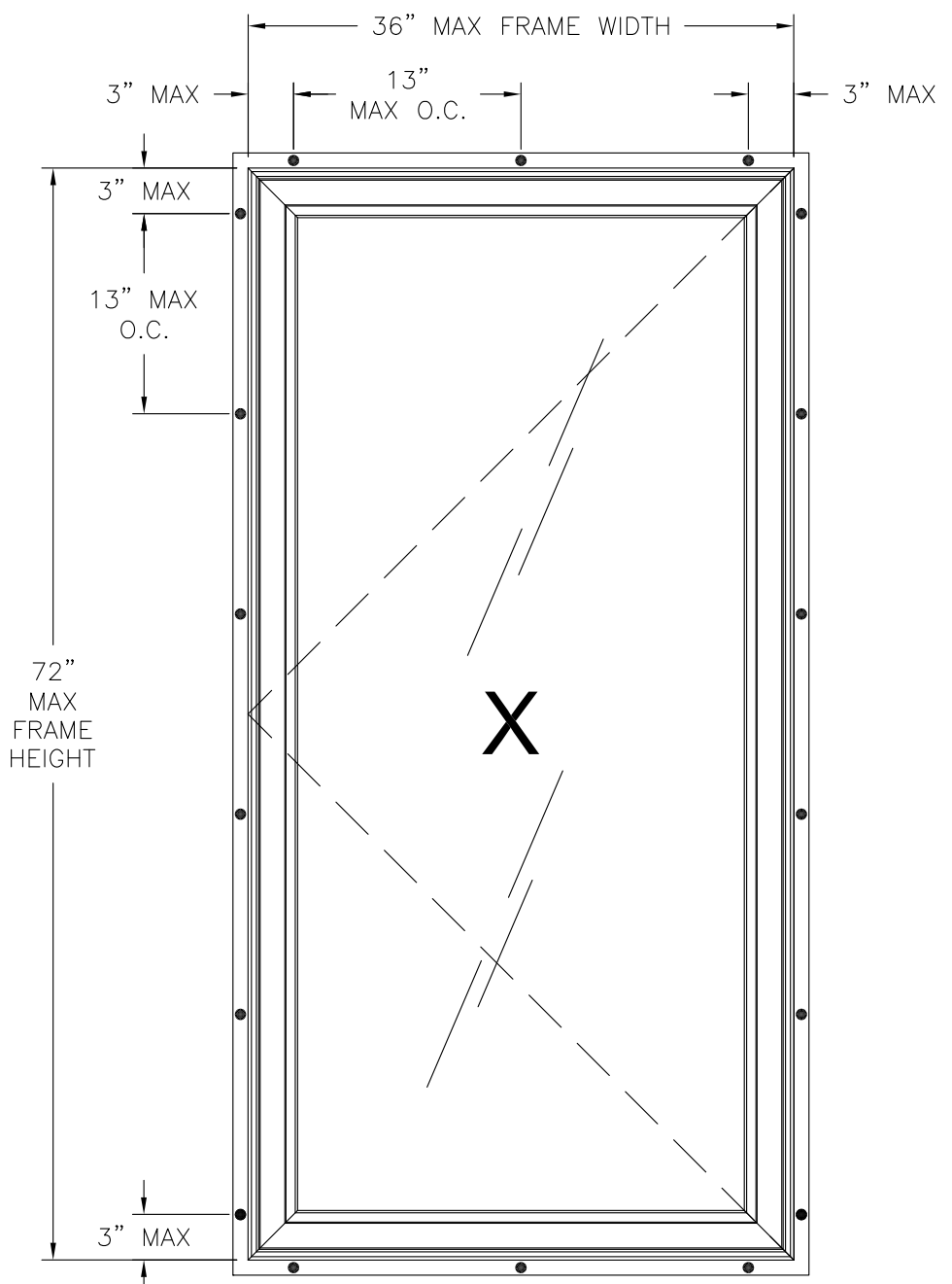
4325 CASEMENT WINDOW EXTERIOR VIEW FIN INSTALLATION
