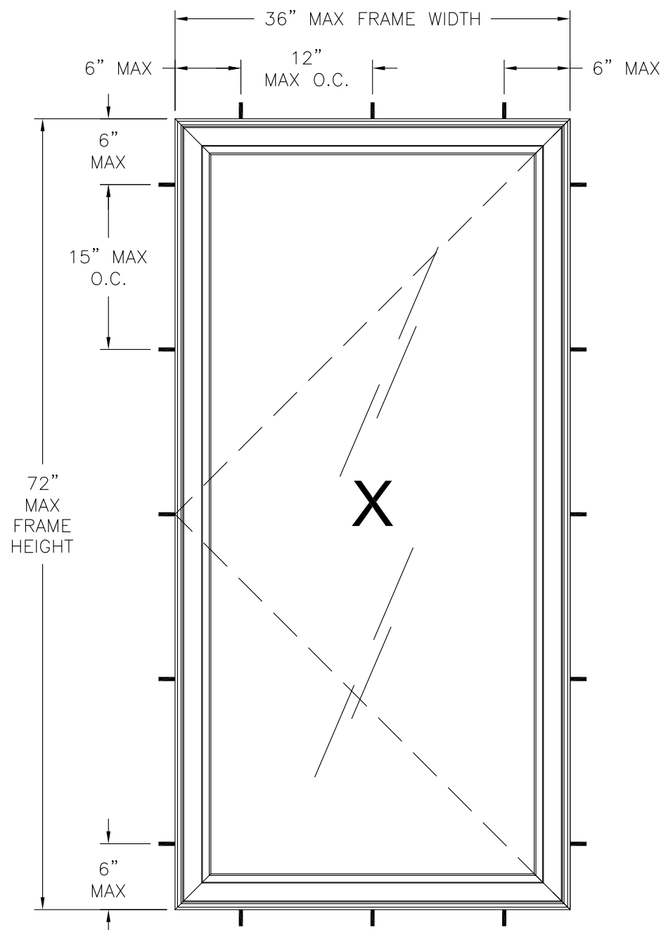
4325 CASEMENT WINDOW EXTERIOR VIEW FRAME INSTALLATION
