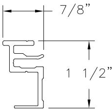
625R1 PERIMETER EXTRUSION ALUMINUM 6063-T6 .063" THICK(MINIMUM)
