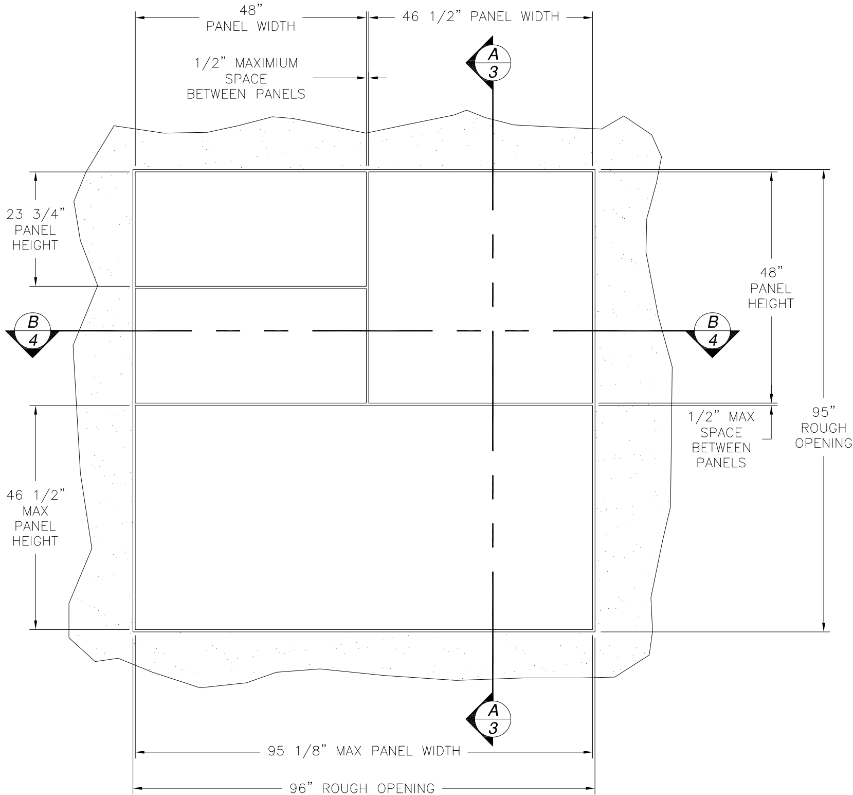
ACM WALL PANEL SYSTEM WET-JOINT EXTERIOR VIEW
