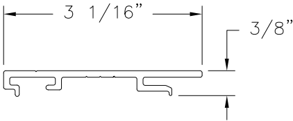
PPC-632 CLIP EXTRUSION ALUMINUM 6063-T6 .100" THICK(MINIMUM)
