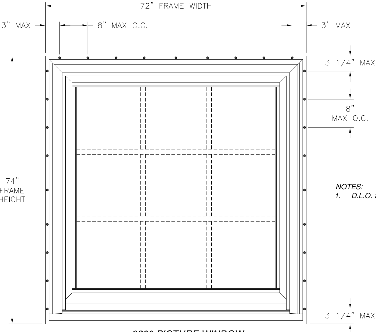
2200 PICTURE WINDOW EXTERIOR VIEW BRICK MOULD INSTALLATION
