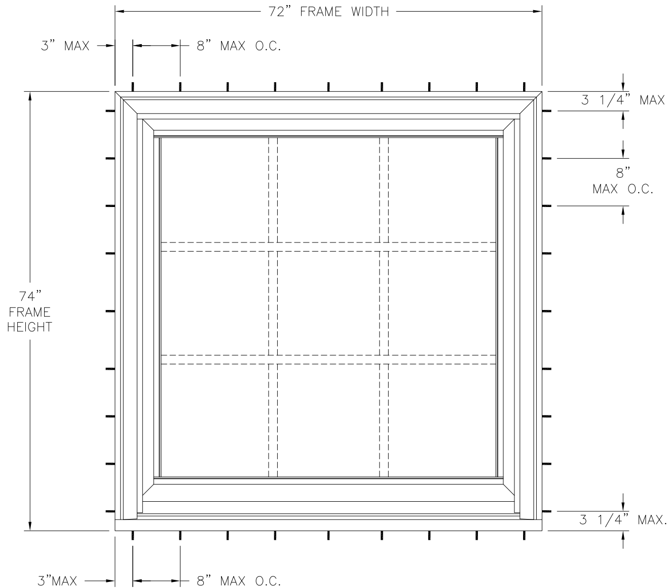
2200 PICTURE WINDOW EXTERIOR VIEW FRAME INSTALLATION
