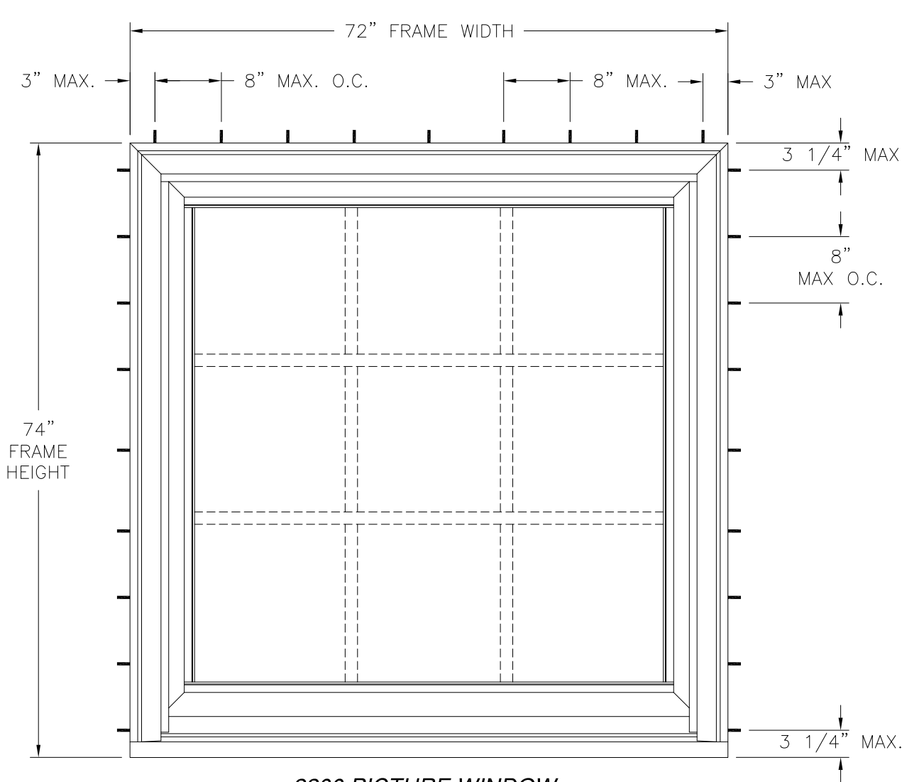
2200 PICTURE WINDOW EXTERIOR VIEW FRAME INSTALLATION
