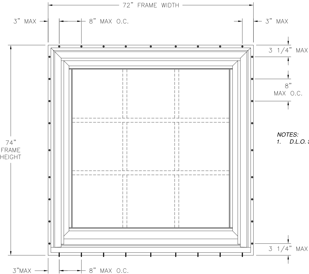
2200 PICTURE WINDOW EXTERIOR VIEW BRICK MOULD INSTALLATION
