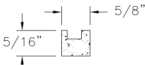
BLIND STOP COMPOSITE (2200-DH-08)
