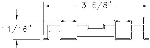
STANDARD LT-100 BALANCE PVC (2200-DH-12)
