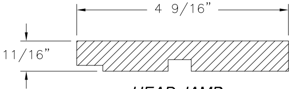
HEAD JAMB WOOD (2200-DH-07)
