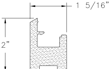
SASH STILE CPVC (2200-DH-17)
