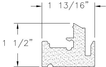
TOP CHECK RAIL CPVC (2200-DH-15)
