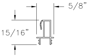
PARTING STOP PVC (2200-DH-13)
