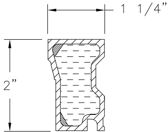
BRICK MOULDING COMPOSITE (2200-DH-10)
