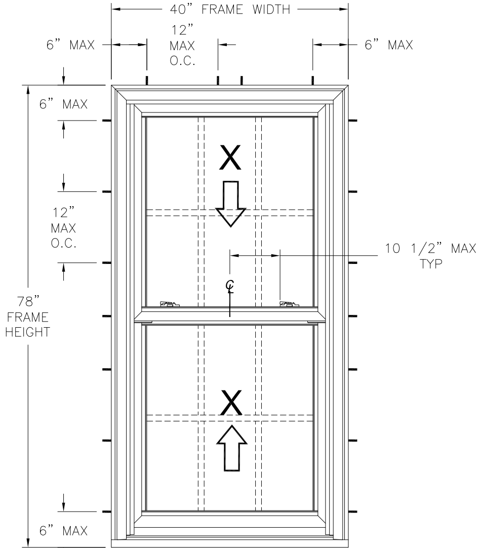
2300 DOUBLE HUNG WINDOW EXTERIOR VIEW FRAME INSTALLATION
