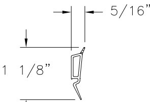
GLAZING BEAD PVC (2300-DH-26)
