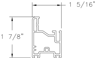
MAIN SASH PVC (2300-DH-17)
