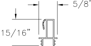
PARTING STOP PVC (2300-DH-13)
