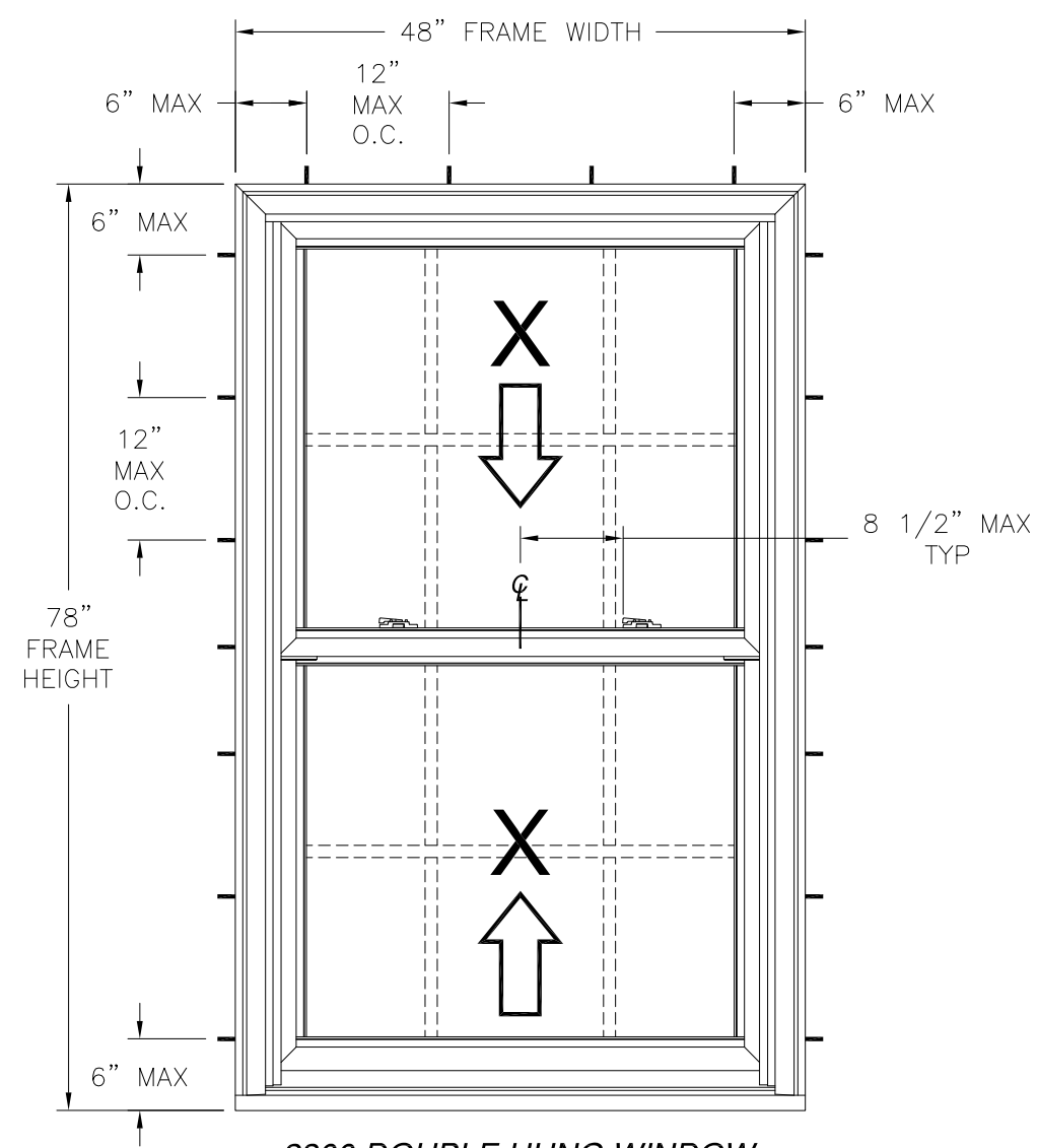
2300 DOUBLE HUNG WINDOW EXTERIOR VIEW FRAME INSTALLATION
