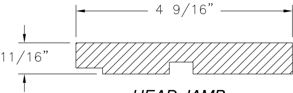
HEAD JAMB WOOD (2300-DH-07)
