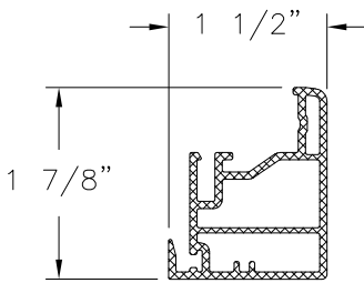
LOCK SASH PVC (2300-DH-15)
