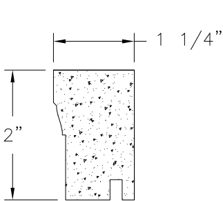
BRICK MOULDING COMPOSITE (2300-DH-10)
