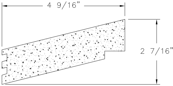
WINDOW SILL COMPOSITE (2300-DH-04)
