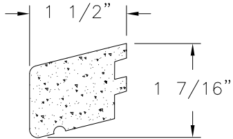
WINDOW SILL NOSE COMPOSITE (2300-DH-05)
