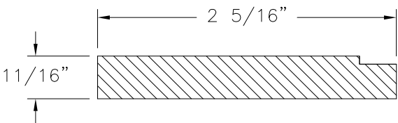
SIDE AND MULLION JAMB WOOD (2300-DH-06)
