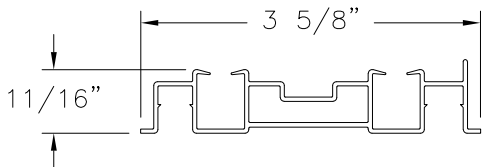
STANDARD LT-100 BALANCE PVC (2300-DH-12)
