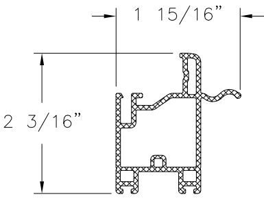
PULL/LIFT SASH PVC (2300-DH-14)
