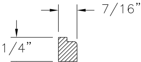
TILT STOP WOOD (2300-DH-09)
