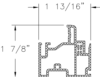
KEEPER SASH PVC (2300-DH-16)
