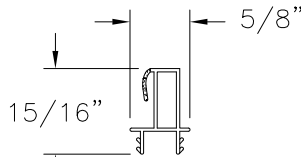
PARTING STOP PVC (2200-DH-13)
