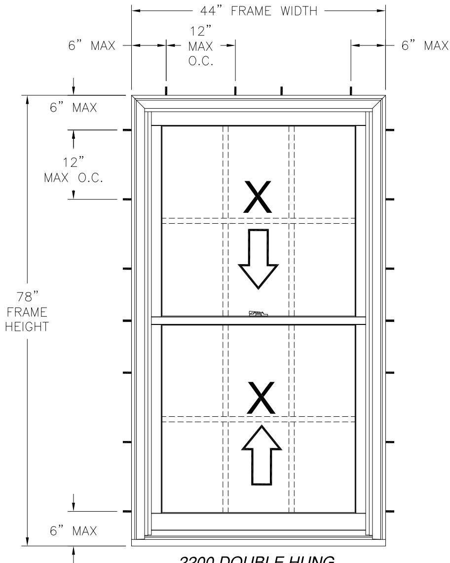
2200 DOUBLE HUNG EXTERIOR VIEW FRAME INSTALLATION
