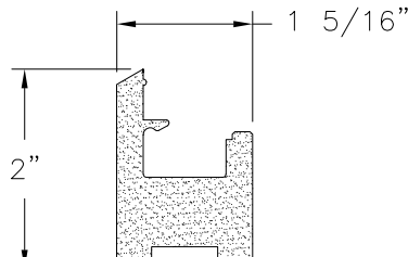
SASH STILE CPVC (2200-DH-17)
