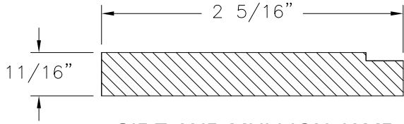
SIDE AND MULLION JAMB WOOD (2200-DH-06)
