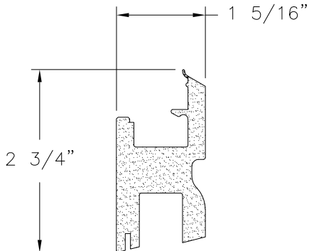
MAIN SASH CPVC (2200-DH-14)
