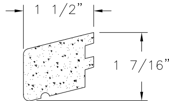
WINDOW SILL NOSE COMPOSITE (2200-DH-05)
