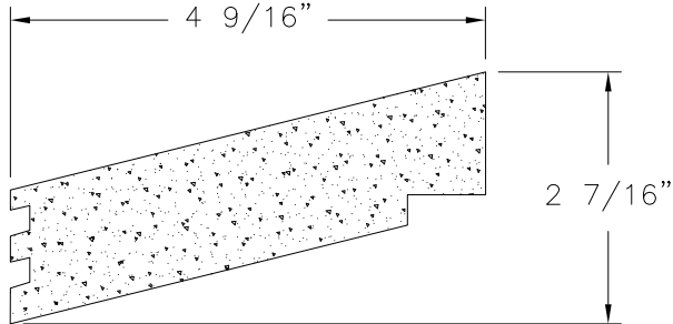
WINDOW SILL COMPOSITE (2200-DH-04)
