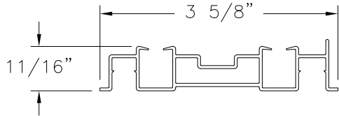
STANDARD LT-100 BALANCE PVC (2200-DH-12)
