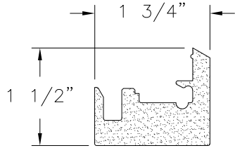
BOTTOM CHECK RAIL CPVC (2200-DH-16)
