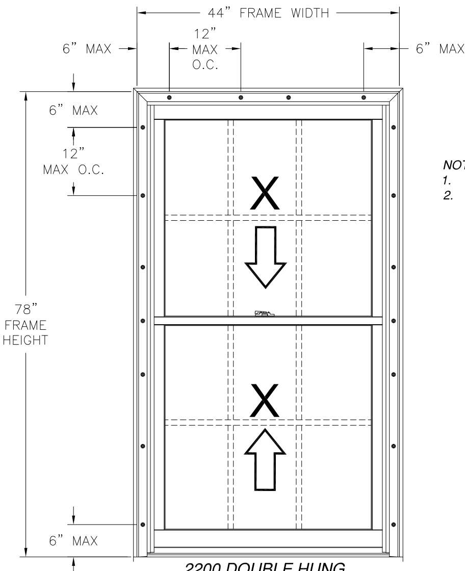
2200 DOUBLE HUNG EXTERIOR VIEW BRICK MOULD INSTALLATION
