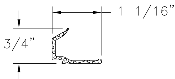
GLAZING BEAD CPVC (2200-DH-18)
