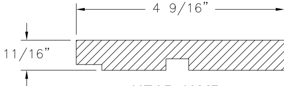
HEAD JAMB WOOD (2200-DH-07)
