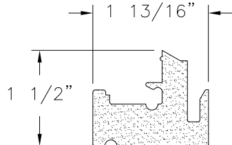
TOP CHECK RAIL CPVC (2200-DH-15)
