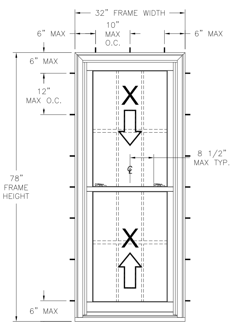
2100 DOUBLE HUNG WINDOW WINDOW EXTERIOR VIEW FRAME INSTALLATION
