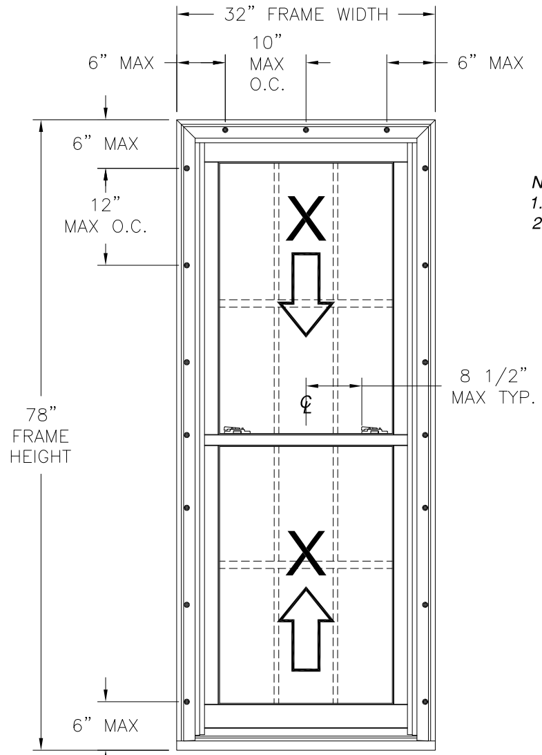
2100 DOUBLE HUNG WINDOW WINDOW EXTERIOR VIEW BRICK MOULD INSTALLATION
