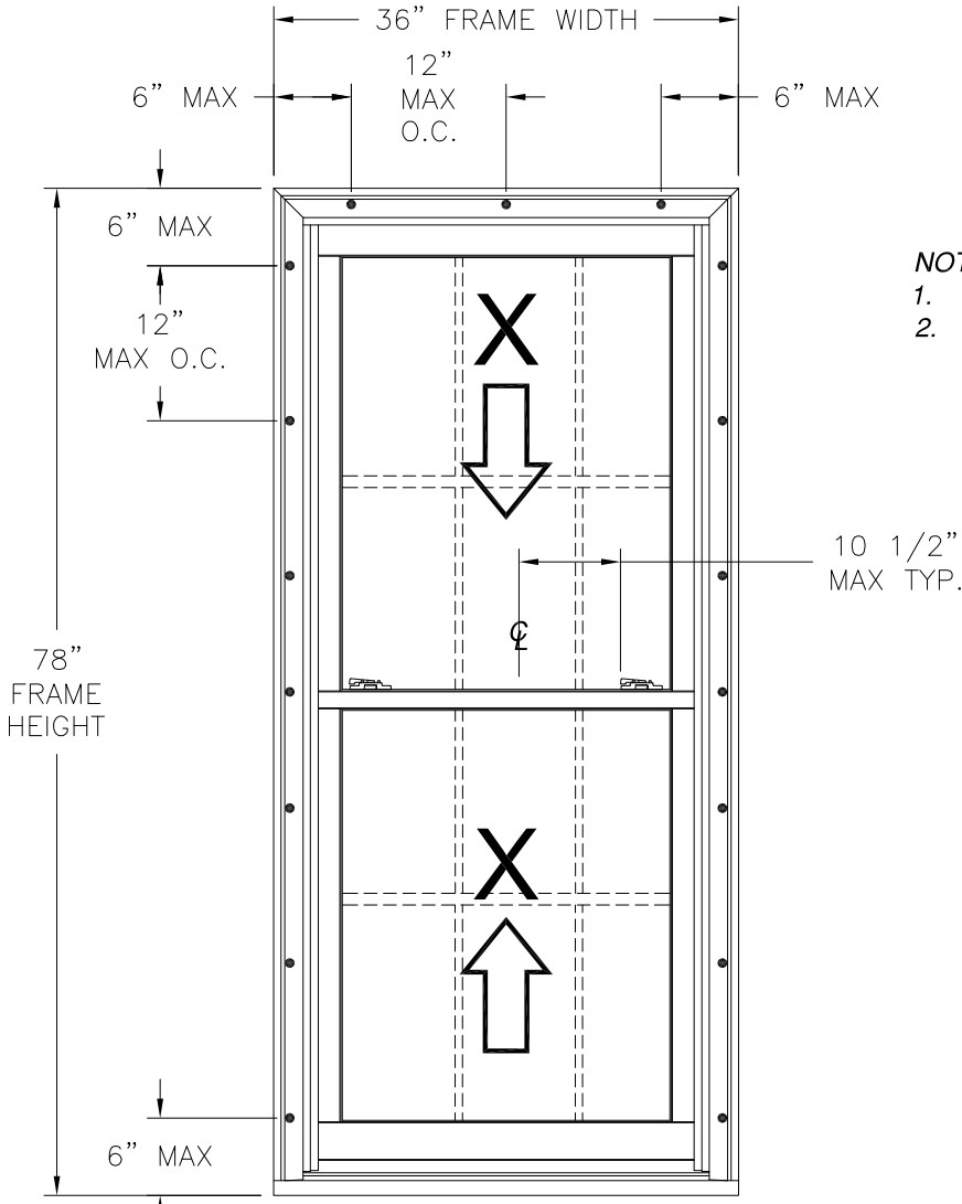
2100 DOUBLE HUNG WINDOW WINDOW EXTERIOR VIEW BRICK MOULD INSTALLATION
