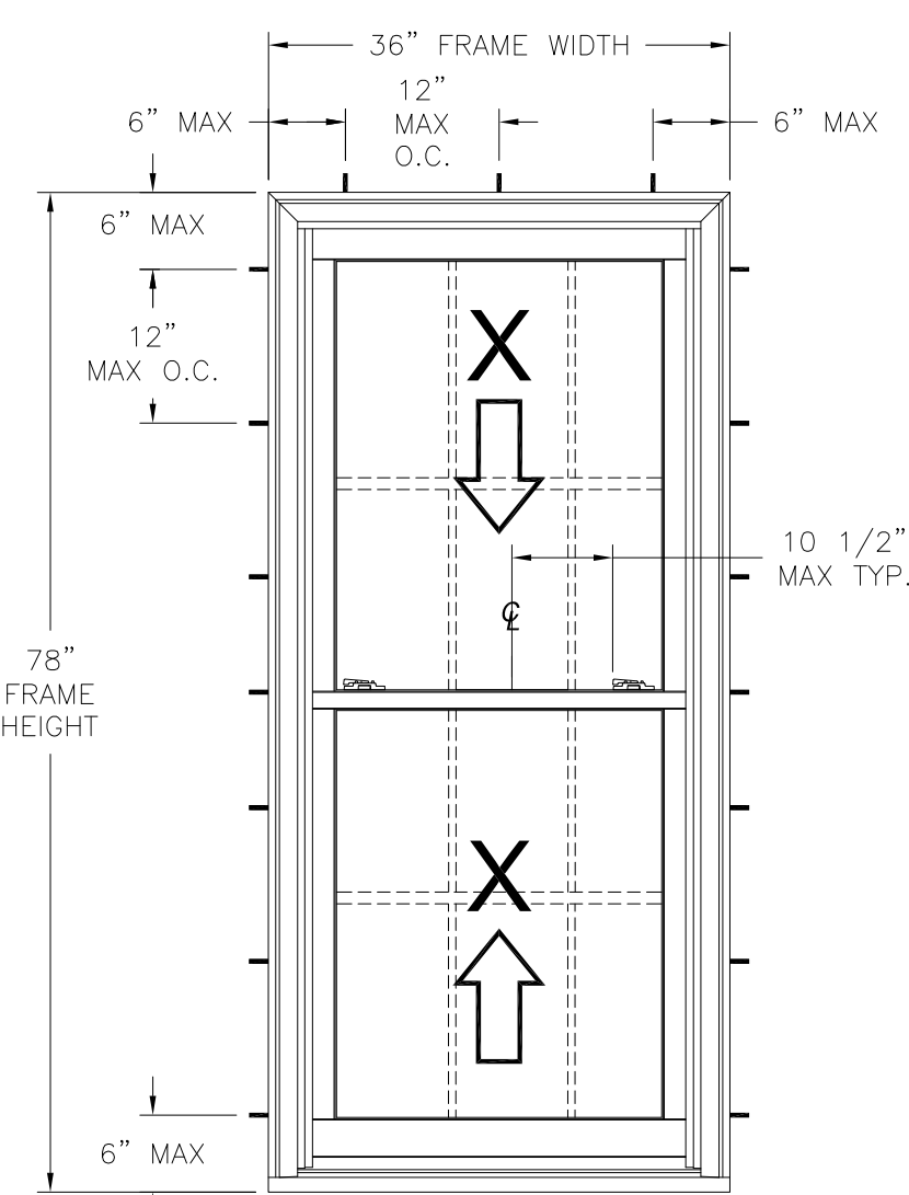
2100 DOUBLE HUNG WINDOW WINDOW EXTERIOR VIEW FRAME INSTALLATION
