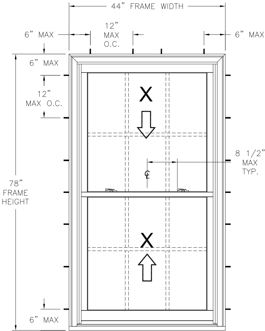
2100 DOUBLE HUNG WINDOW WINDOW EXTERIOR VIEW FRAME INSTALLATION
