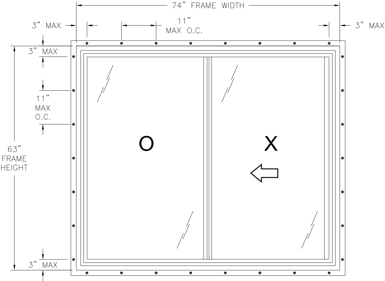
SECURITY SERIES 6050 HS WINDOW EXTERIOR VIEW FIN INSTALLATION
