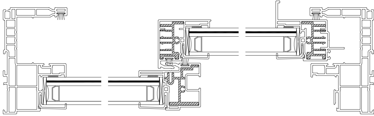
HORIZONTAL CROSS SECTION FINLESS FRAME
