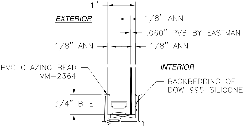
GLAZING DETAIL
