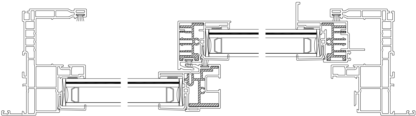
HORIZONTAL CROSS SECTION FLANGE FRAME
