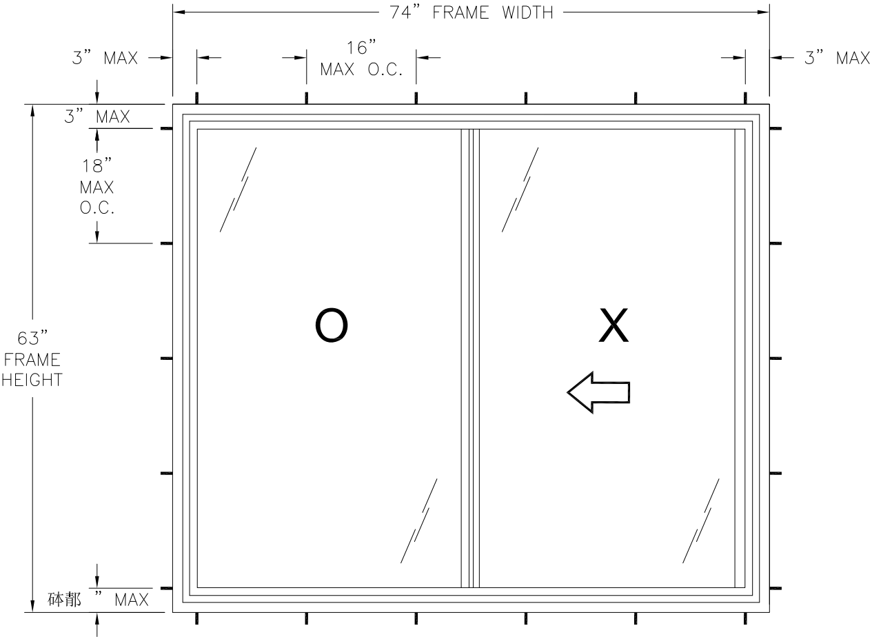
SECURITY SERIES 6050 HS WINDOW EXTERIOR VIEW FINLESS AND FLANGE INSTALLATION
