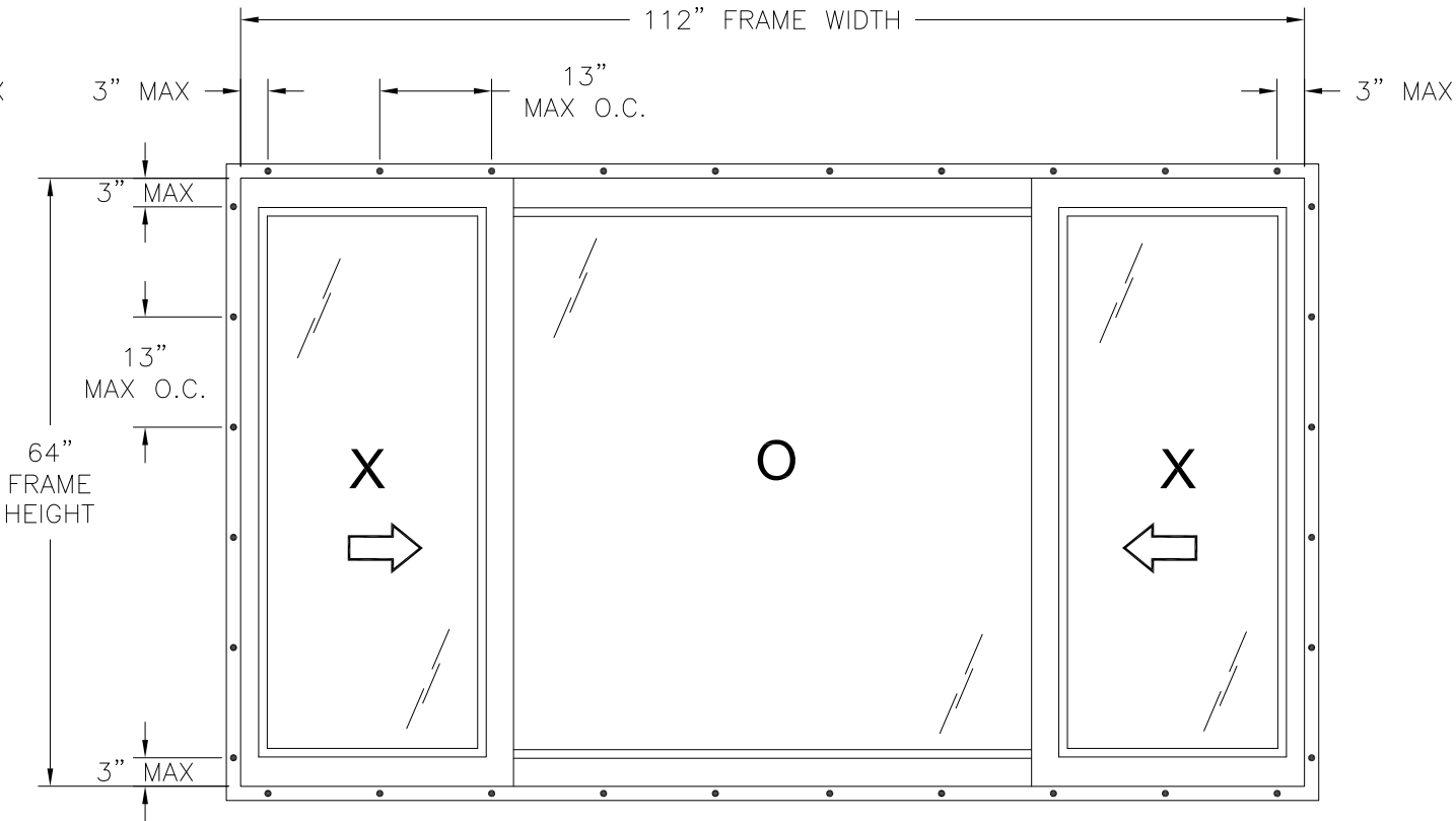
SERIES 9050 VINYL HS WINDOW EXTERIOR VIEW FIN INSTALLATION
