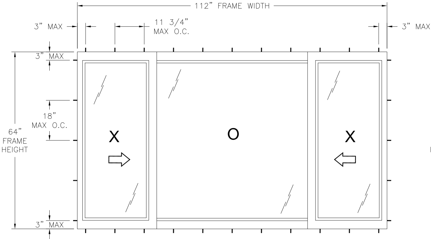
SERIES 9050 VINYL HS WINDOW EXTERIOR VIEW FRAME INSTALLATION
