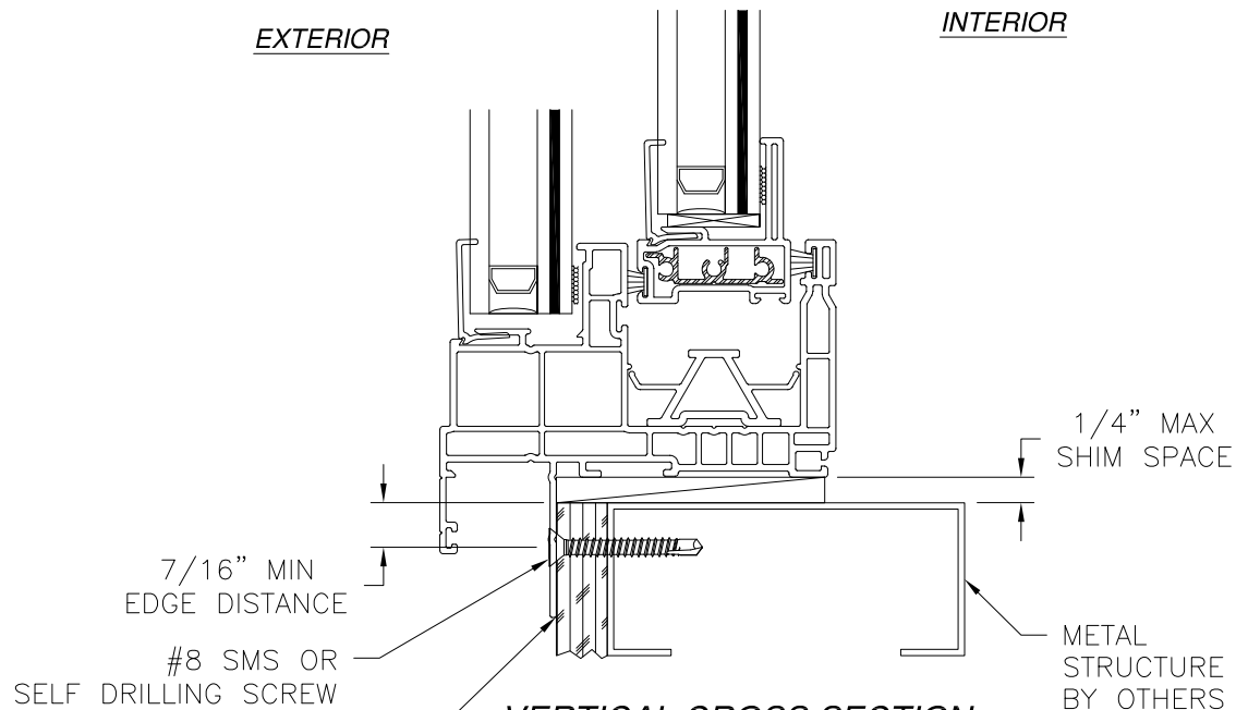
VERTICAL CROSS SECTION METAL STRUCTURE INSTALLATION
