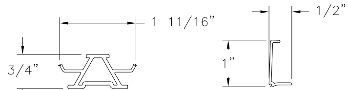
TRACK (VM-2372) PVC
