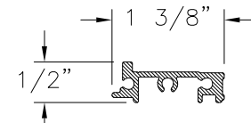
SASH REINFORCEMENT (T-11211) ALUMINUM
