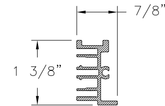
MEETING RAIL REINFORCEMENT (T-11222) ALUMINUM
