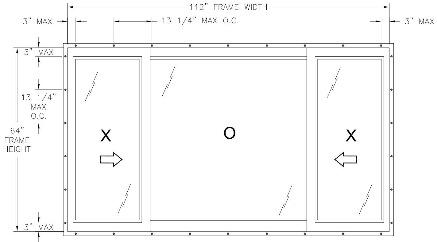
SERIES 9050 HS WINDOW EXTERIOR VIEW FIN INSTALLATION
