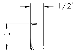
BEAD (VM-2365) PVC
