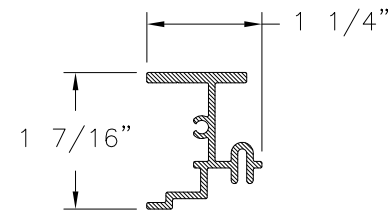
STILE REINFORCEMENT (T-11333) ALUMINUM
