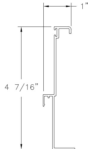
2" SILL RISER ALUMINUM
