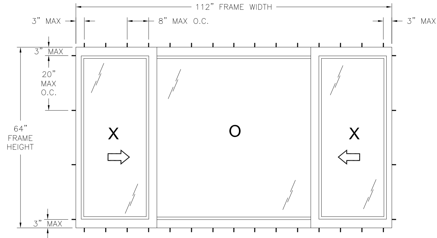
SERIES 9050 HS WINDOW EXTERIOR VIEW FRAME INSTALLATION
