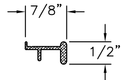
REINFORCEMENT 058288 ALUMINUM 6063-T5 .060" THICK
