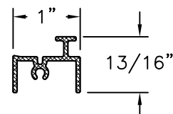
REINFORCEMENT 058287 ALUMINUM 6063-T5 .060" THICK
