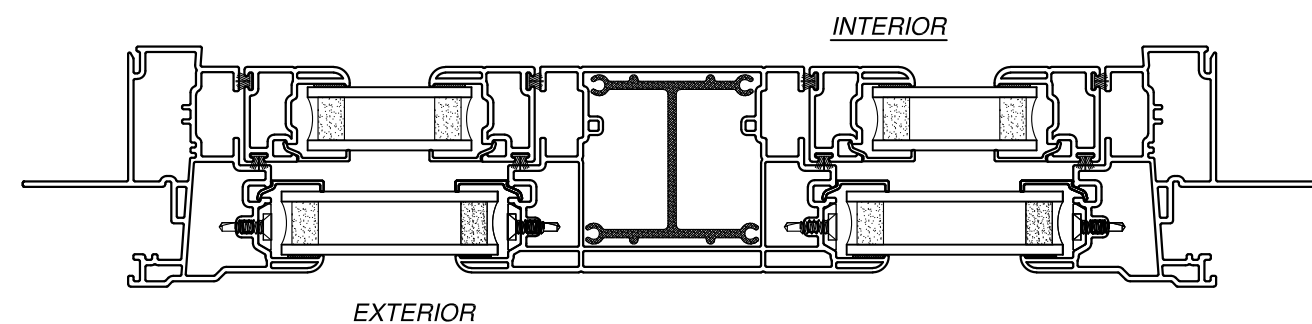
HORIZONTAL CROSS SECTION
