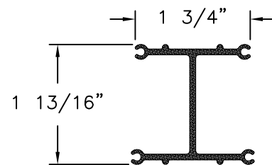
REINFORCEMENT 058286 GALVANIZED STEEL .075" THICK
