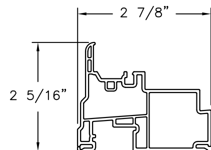
FIXED FRAME PVC .065" THICK
