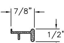
REINFORCEMENT T-11820 ALUMINUM 6063-T5 .060" THICK
