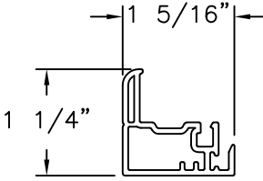
INTERIOR SASH PVC .065" THICK
