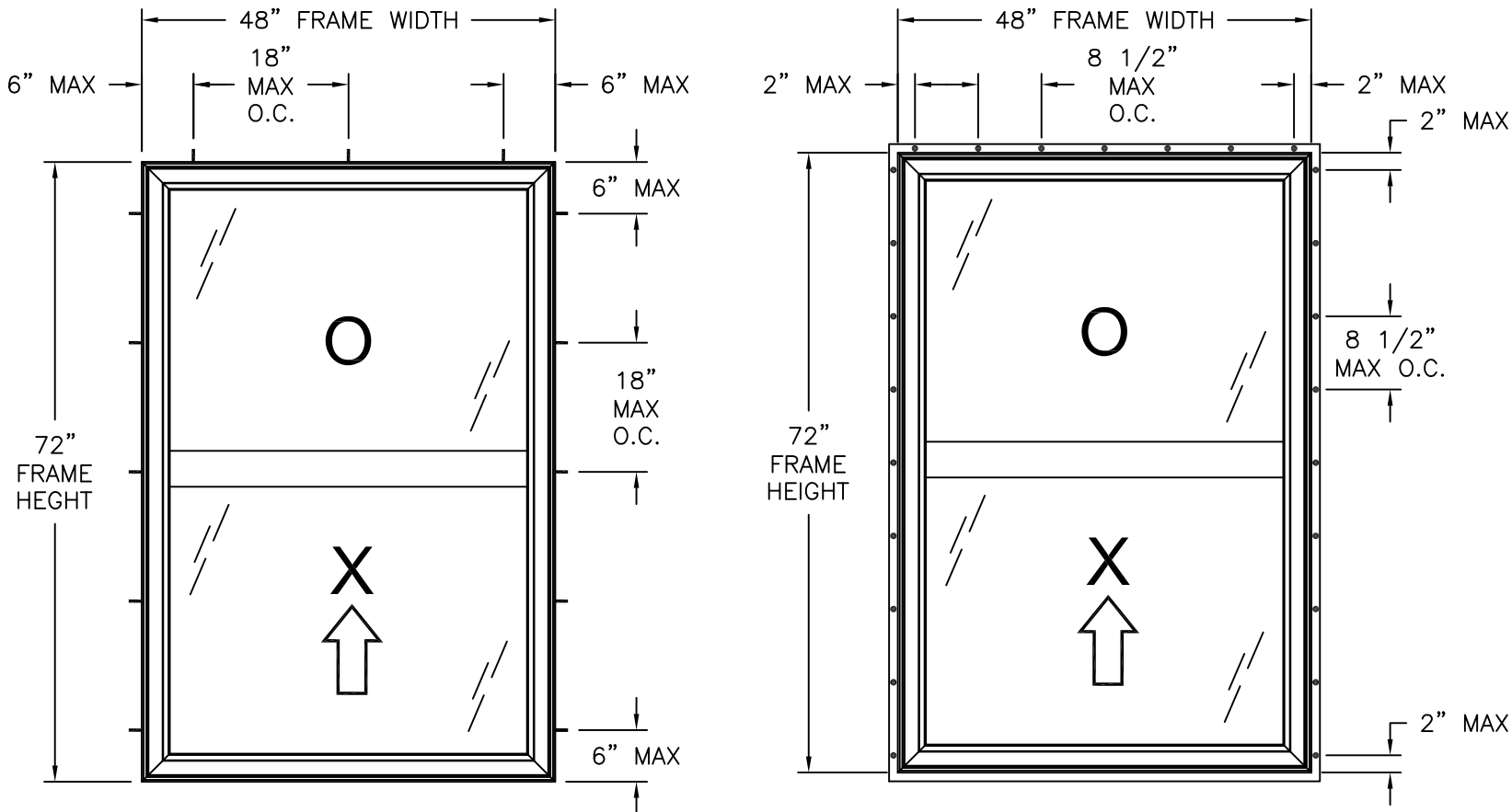
400 VINYL SINGLE HUNG WINDOW EXTERIOR VIEW FRAME INSTALLATION
