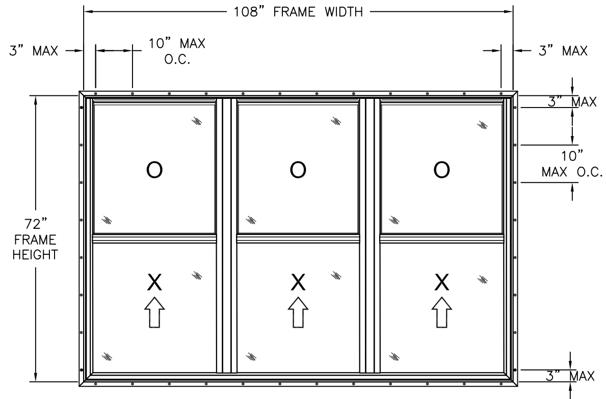
400 VINYL TRIPLE SINGLE HUNG WINDOW EXTERIOR VIEW FIN INSTALLATION
