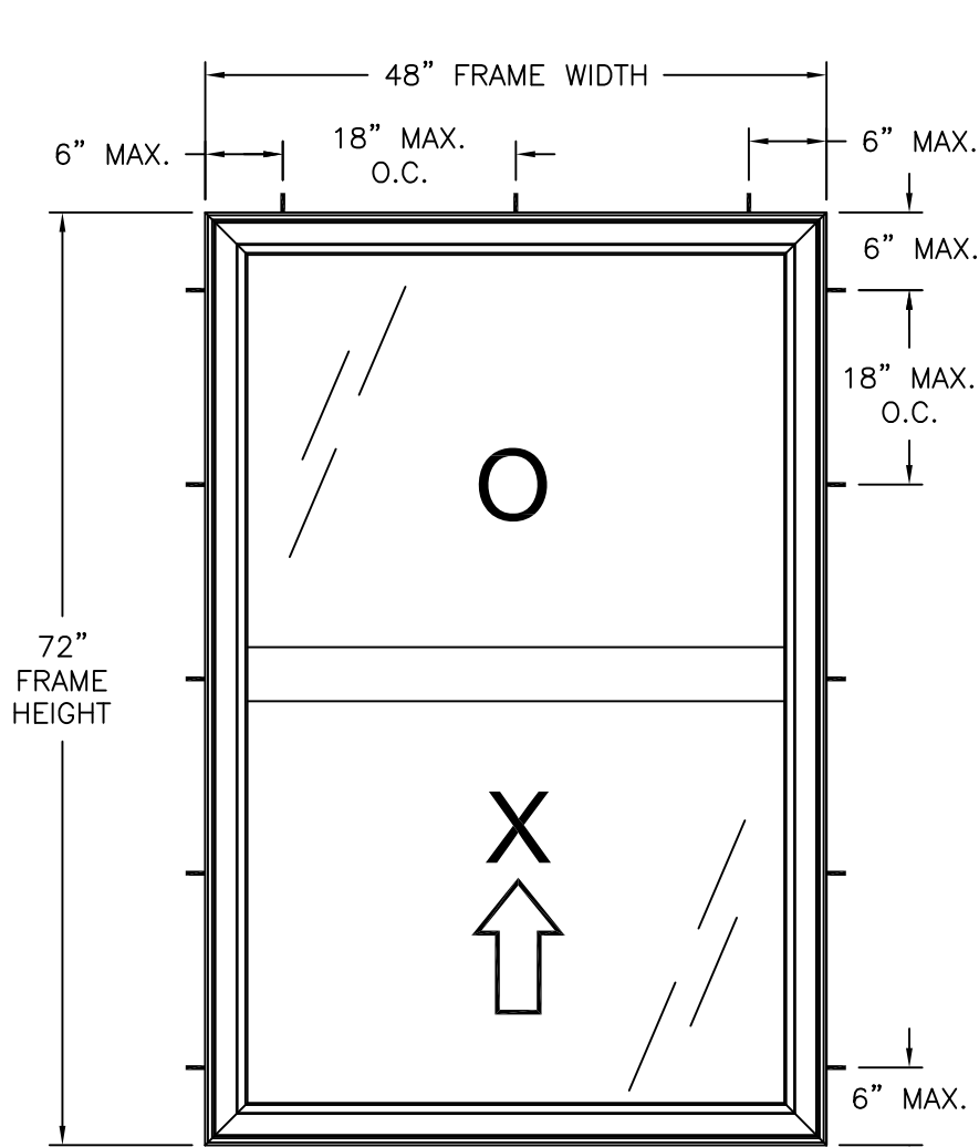
400 VINYL SINGLE HUNG WINDOW EXTERIOR VIEW FRAME INSTALLATION
