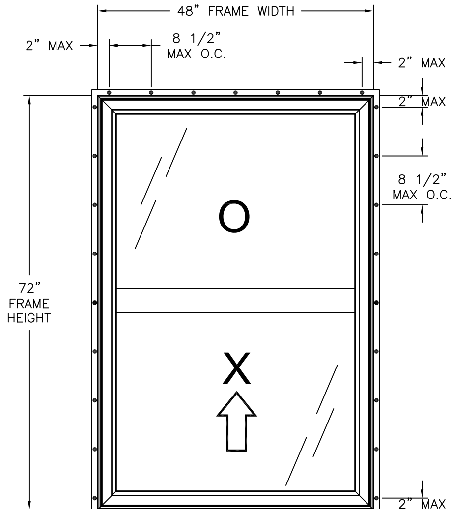
400 VINYL SINGLE HUNG WINDOW EXTERIOR VIEW FIN INSTALLATION
