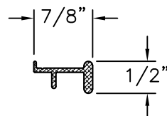
REINFORCEMENT T-11820 ALUMINUM 6063-T5 .060" THICK
