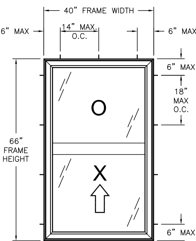
400 VINYL SINGLE HUNG WINDOW EXTERIOR VIEW FRAME INSTALLATION
