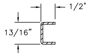
REINFORCEMENT ST-1791A GALVANIZED STEEL .075" THICK
