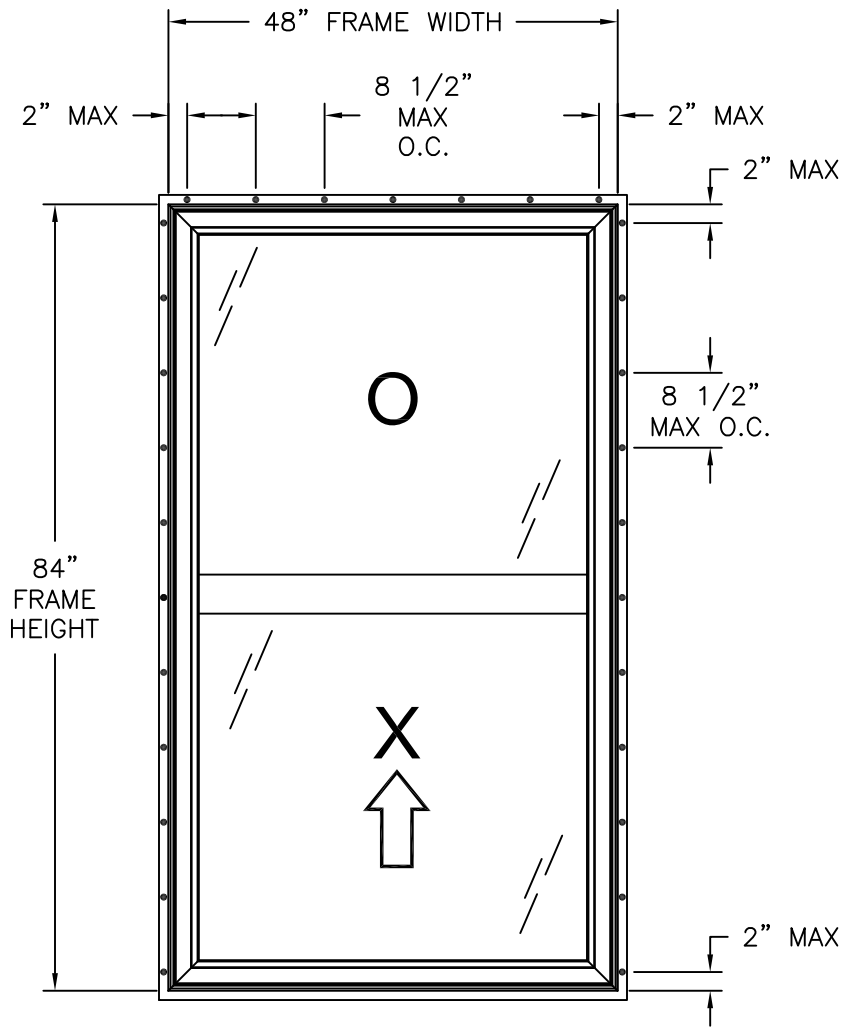
400 VINYL SINGLE HUNG WINDOW EXTERIOR VIEW FIN INSTALLATION
