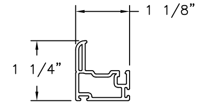
MAIN SASH PVC .065" THICK
