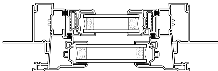
HORIZONTAL CROSS SECTION
