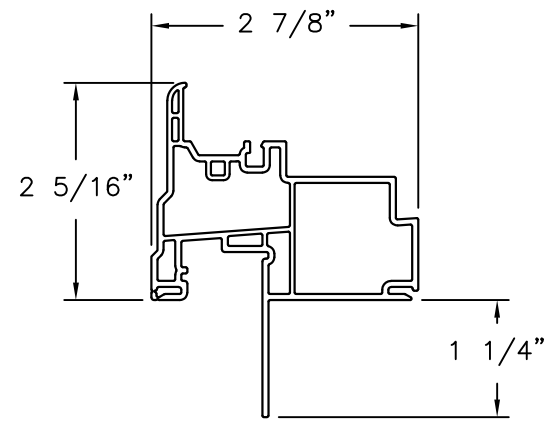
FIXED FRAME PVC .065" THICK
