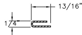
REINFORCEMENT ST-1789A GALVANIZED STEEL .060" THICK
