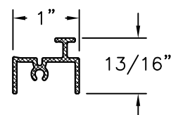
REINFORCEMENT T-11974 ALUMINUM 6063-T5 .060" THICK
