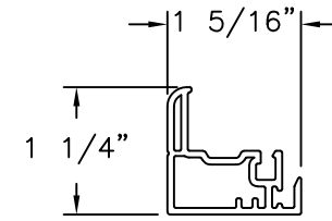
INTERIOR SASH PVC .065" THICK
