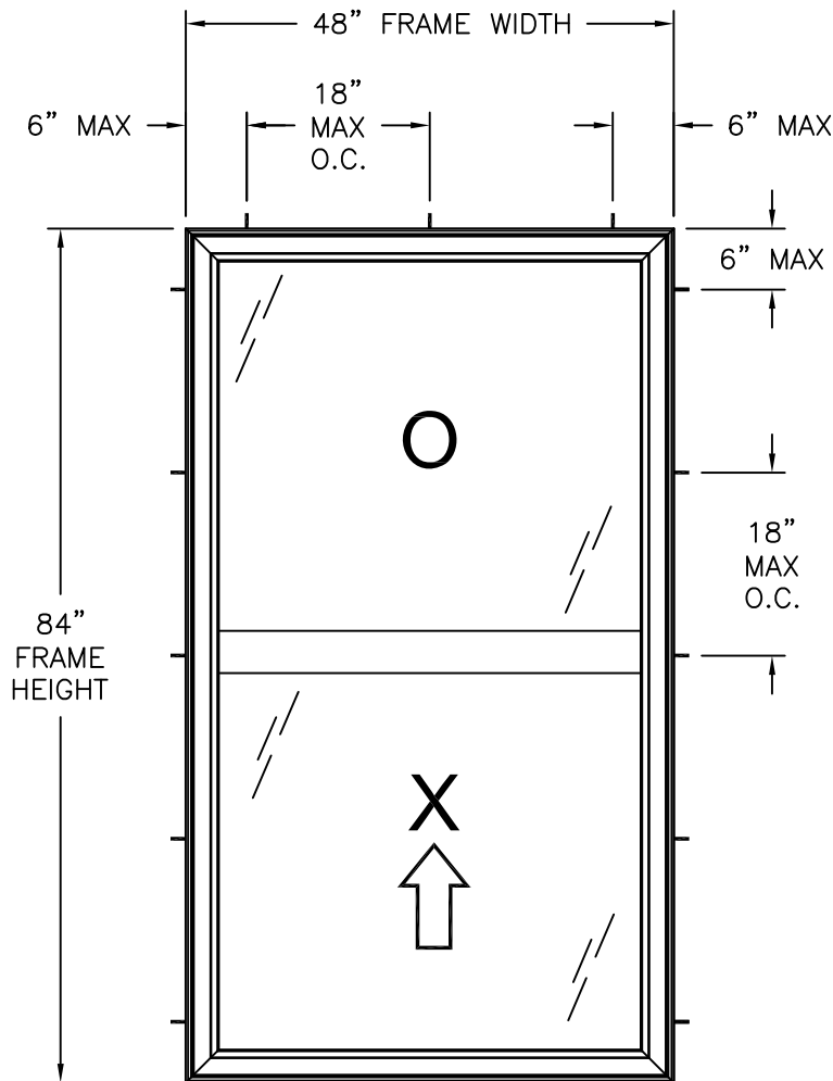
400 VINYL SINGLE HUNG WINDOW EXTERIOR VIEW FRAME INSTALLATION
