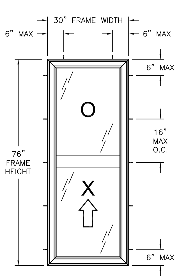
400 VINYL SINGLE HUNG WINDOW EXTERIOR VIEW FRAME INSTALLATION
