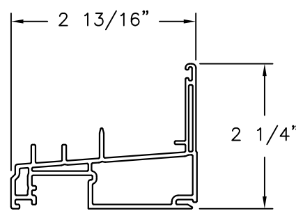
SILL FRAME PVC .065" THICK
