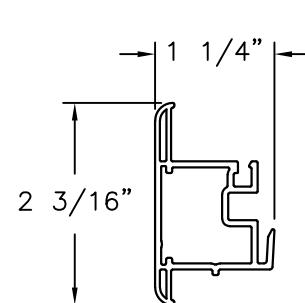
OX BAR PVC .065" THICK
