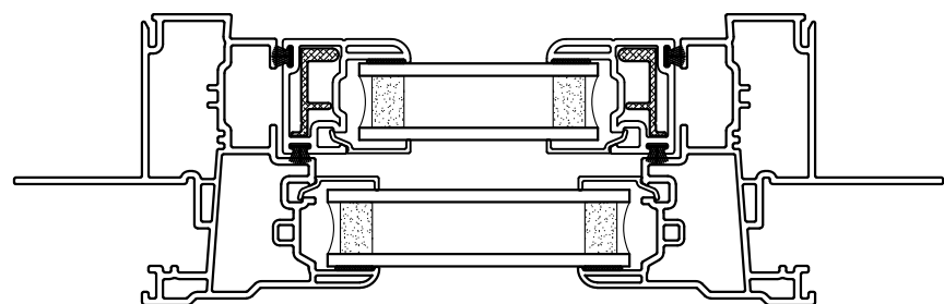
HORIZONTAL CROSS SECTION
