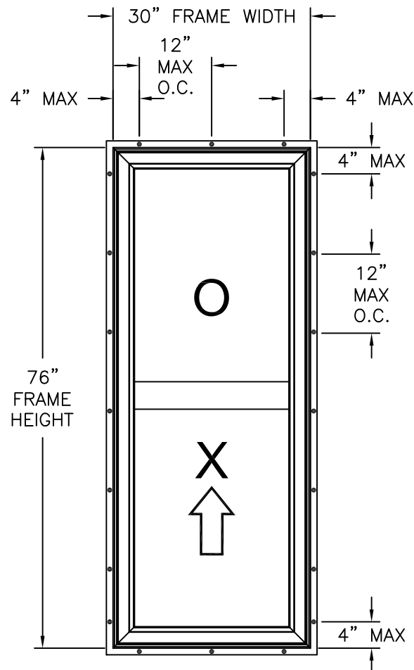
400 VINYL SINGLE HUNG WINDOW EXTERIOR VIEW FIN INSTALLATION
