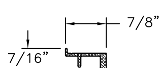
REINFORCEMENT T-12576 ALUMINUM 6063-T5 .060" THICK
