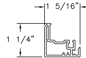
INTERIOR SASH PVC .065" THICK
