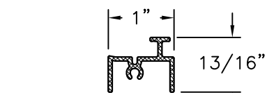
REINFORCEMENT T-11974 ALUMINUM 6063-T5 .060" THICK
