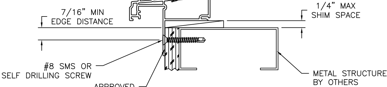
VERTICAL CROSS SECTION METAL STRUCTURE INSTALLATION
