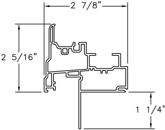
JAMB FRAME PVC .065" THICK
