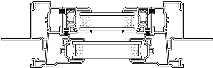
SH HORIZONTAL CROSS SECTION
