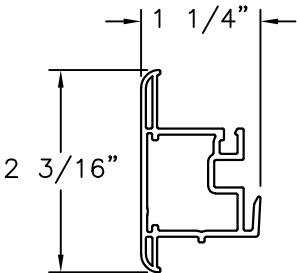
OX BAR PVC .065" THICK
