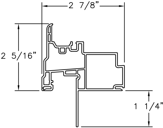
FIXED FRAME PVC .065" THICK
