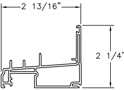
SILL FRAME PVC .065" THICK
