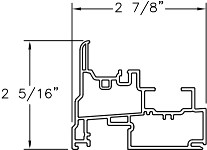
JAMB FRAME PVC .065" THICK
