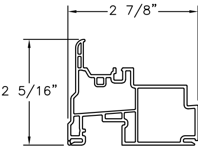
FIXED FRAME PVC .065" THICK
