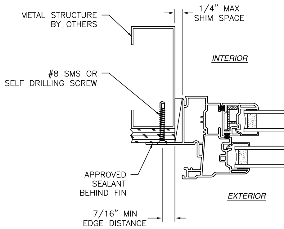
JAMB INSTALLATION DETAIL METAL STRUCTURE INSTALLATION SINGLE HUNG SHOWN, TRANSOM SIMILAR
