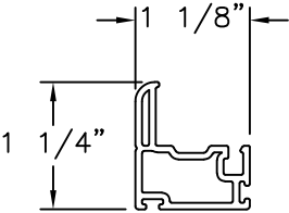
MAIN SASH PVC .065" THICK
