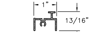
REINFORCEMENT 058287 ALUMINUM 6063-T5 .060" THICK
