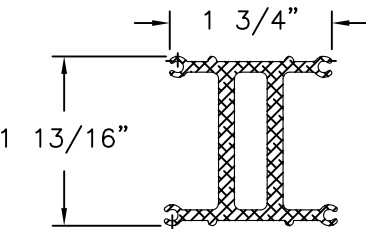
REINFORCEMENT 058328 ALUMINUM 6063-T5 .125" THICK
