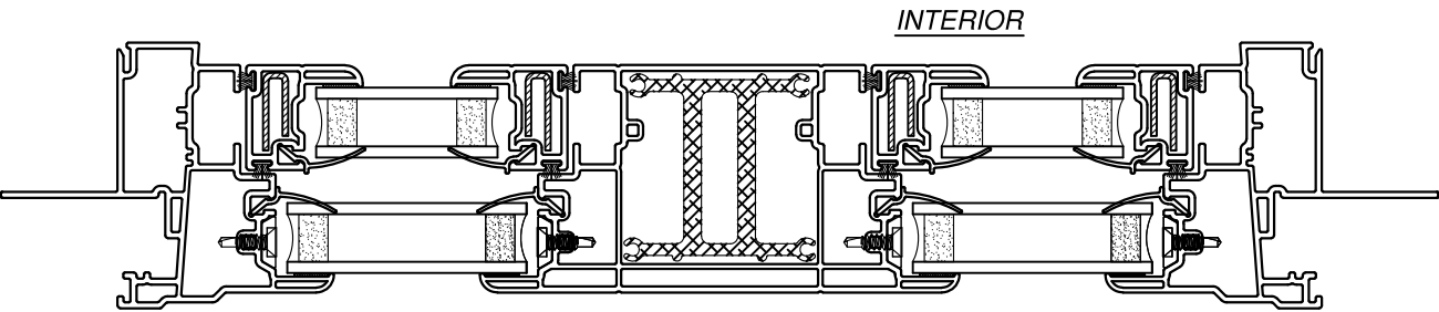
HORIZONTAL CROSS SECTION
