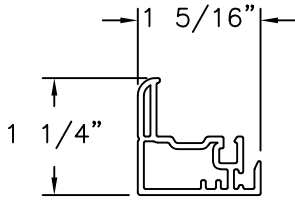
INTERLOCK SASH PVC .065" THICK
