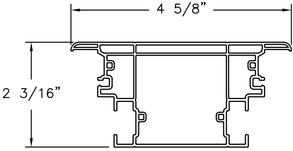
COMMON MULLION PVC .065" THICK
