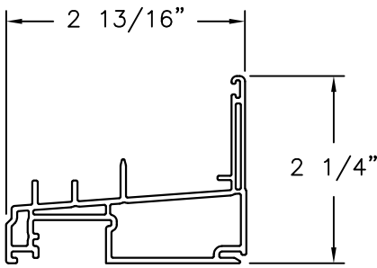
SILL FRAME PVC .065" THICK
