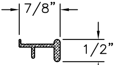
REINFORCEMENT 058288 ALUMINUM 6063-T5 .060" THICK
