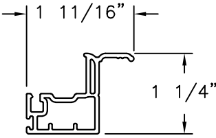
SILL SASH PVC .065" THICK
