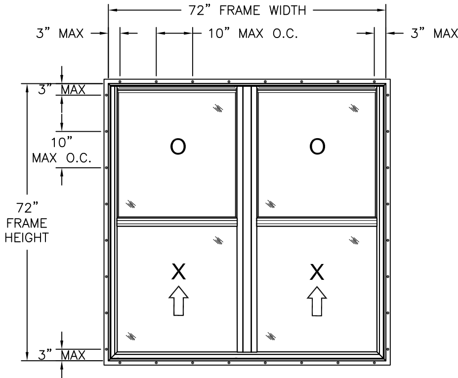
400 VINYL TWIN SINGLE HUNG WINDOW EXTERIOR VIEW FIN INSTALLATION
