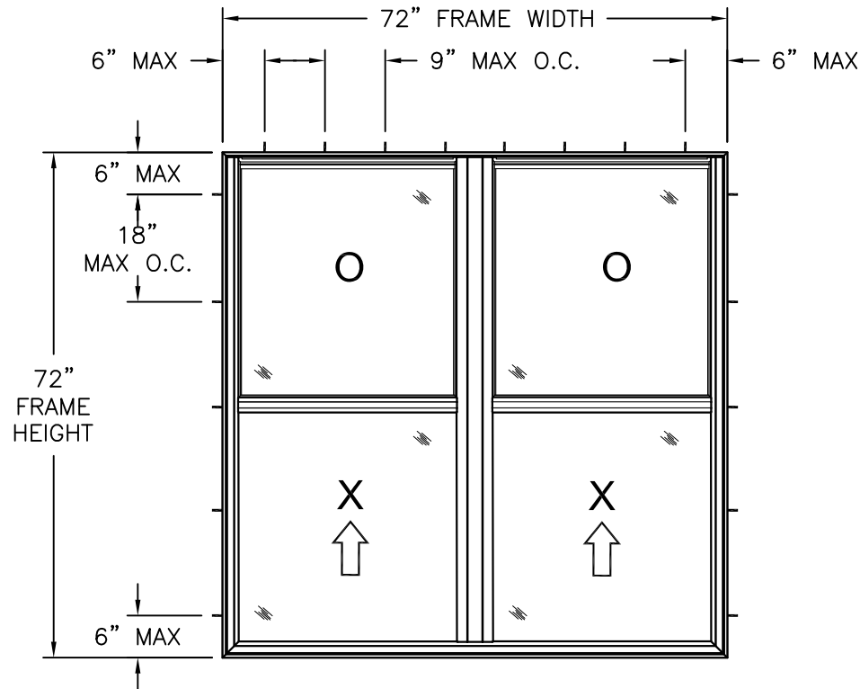
400 VINYL TWIN SINGLE HUNG WINDOW EXTERIOR VIEW FRAME INSTALLATION
