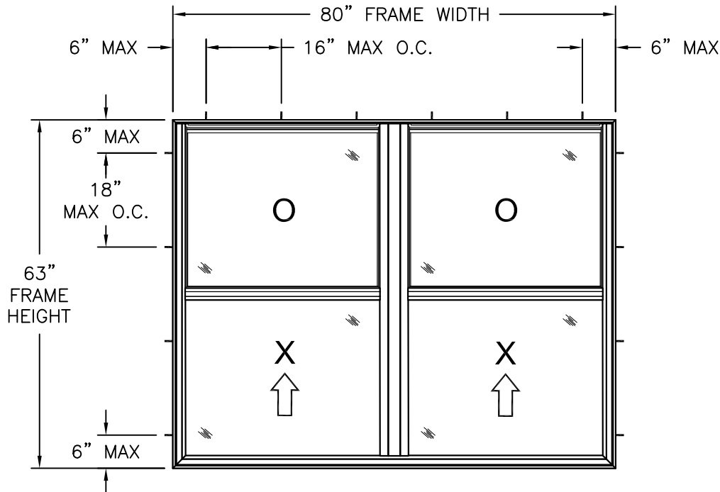
400 VINYL TWIN SINGLE HUNG WINDOW EXTERIOR VIEW FRAME INSTALLATION
