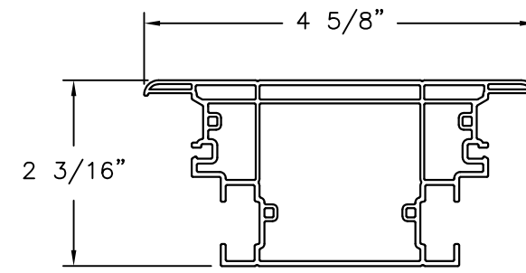
COMMON MULLION PVC .065" THICK
