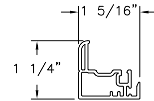
INTERLOCK SASH PVC .065" THICK
