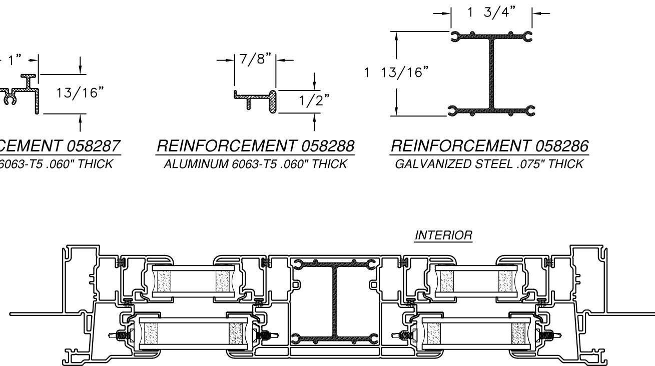
HORIZONTAL CROSS SECTION
