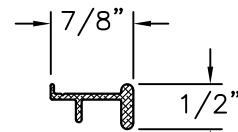
REINFORCEMENT 058288 ALUMINUM 6063-T5 .060" THICK
