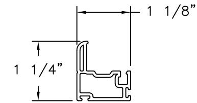
MAIN SASH PVC .065" THICK
