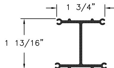
REINFORCEMENT 058286 GALVANIZED STEEL .075" THICK
