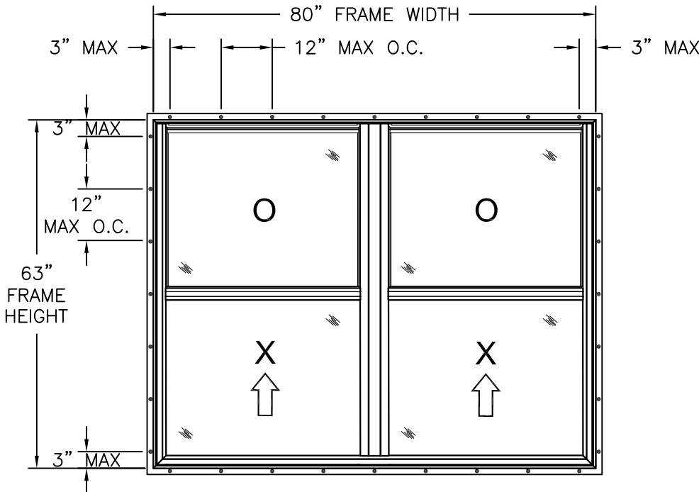
400 VINYL TWIN SINGLE HUNG WINDOW EXTERIOR VIEW FIN INSTALLATION
