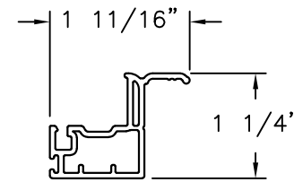
SILL SAH PVC .065" THICK
