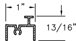
REINFORCEMENT 058287 ALUMINUM 6063-T5 .060" THICK
