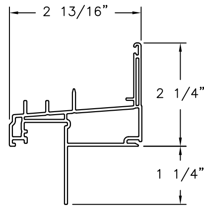
SILL FRAME PVC .065" THICK
