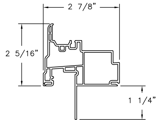
FIXED FRAME PVC .065" THICK
