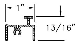
REINFORCEMENT T-11974 ALUMINUM 6063-T5 .060" THICK
