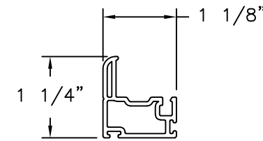
MAIN SASH PVC .065" THICK
