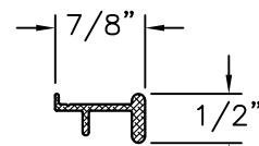
REINFORCEMENT T-11820 ALUMINUM 6063-T5 .060" THICK
