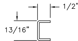
REINFORCEMENT ST-1791A GALVANIZED STEEL .075" THICK
