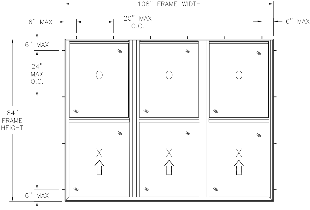
400 TRIPLE SINGLE HUNG WINDOW EXTERIOR VIEW FRAME INSTALLATION
