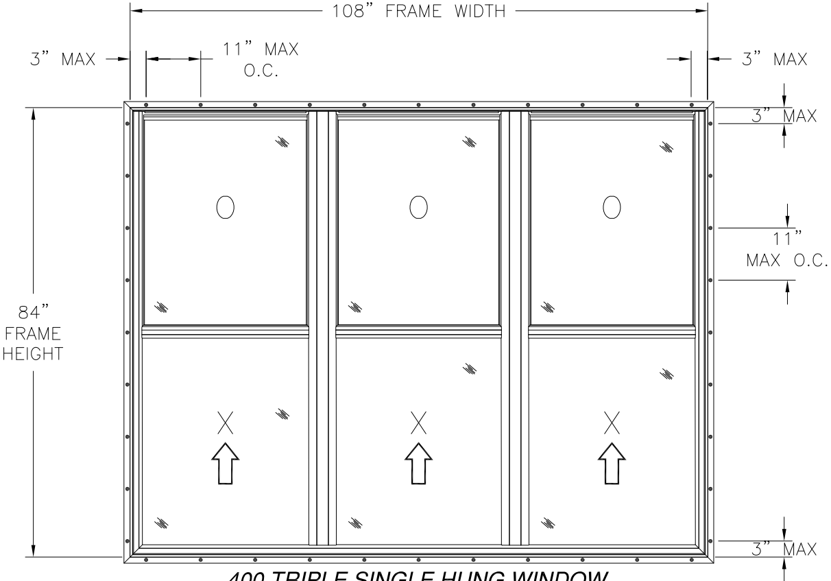
400 TRIPLE SINGLE HUNG WINDOW EXTERIOR VIEW FIN INSTALLATION
