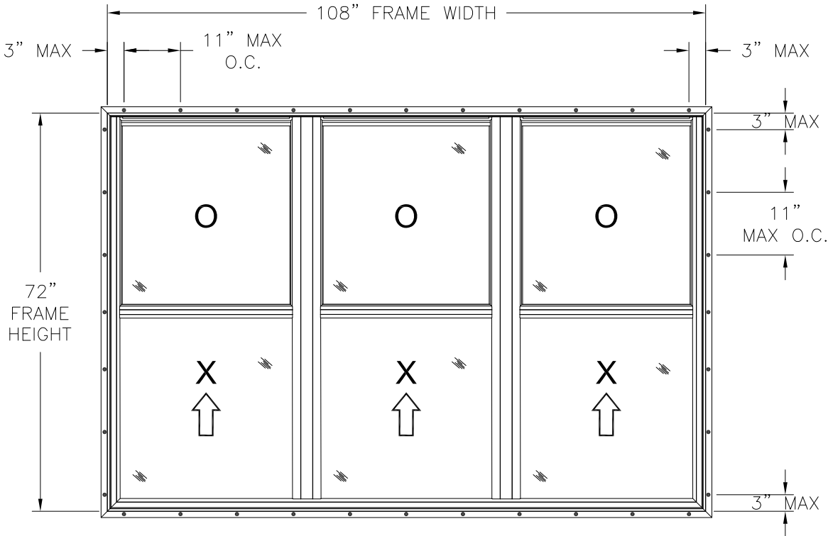
400 VINYL TRIPLE SINGLE HUNG WINDOW EXTERIOR VIEW FIN INSTALLATION
