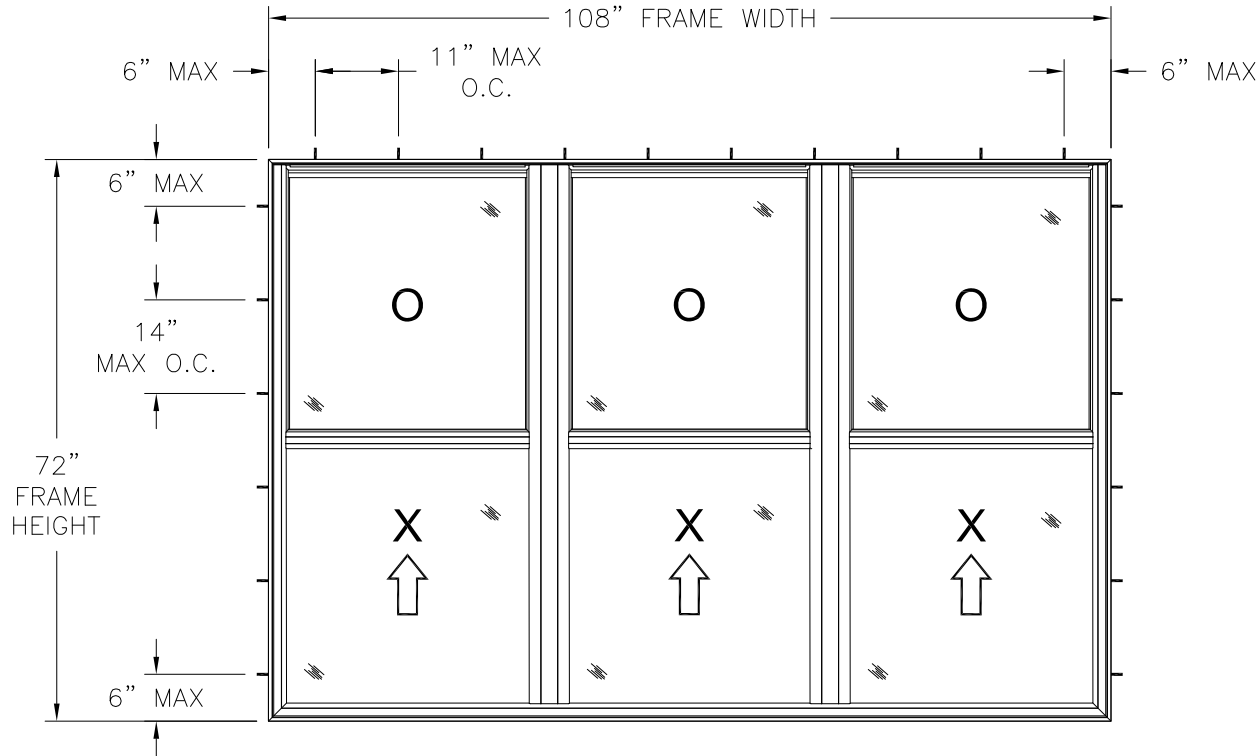
400 VINYL TRIPLE SINGLE HUNG WINDOW EXTERIOR VIEW FRAME INSTALLATION
