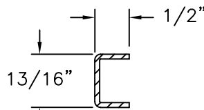
REINFORCEMENT ST-1791A GALVANIZED STEEL .075" THICK
