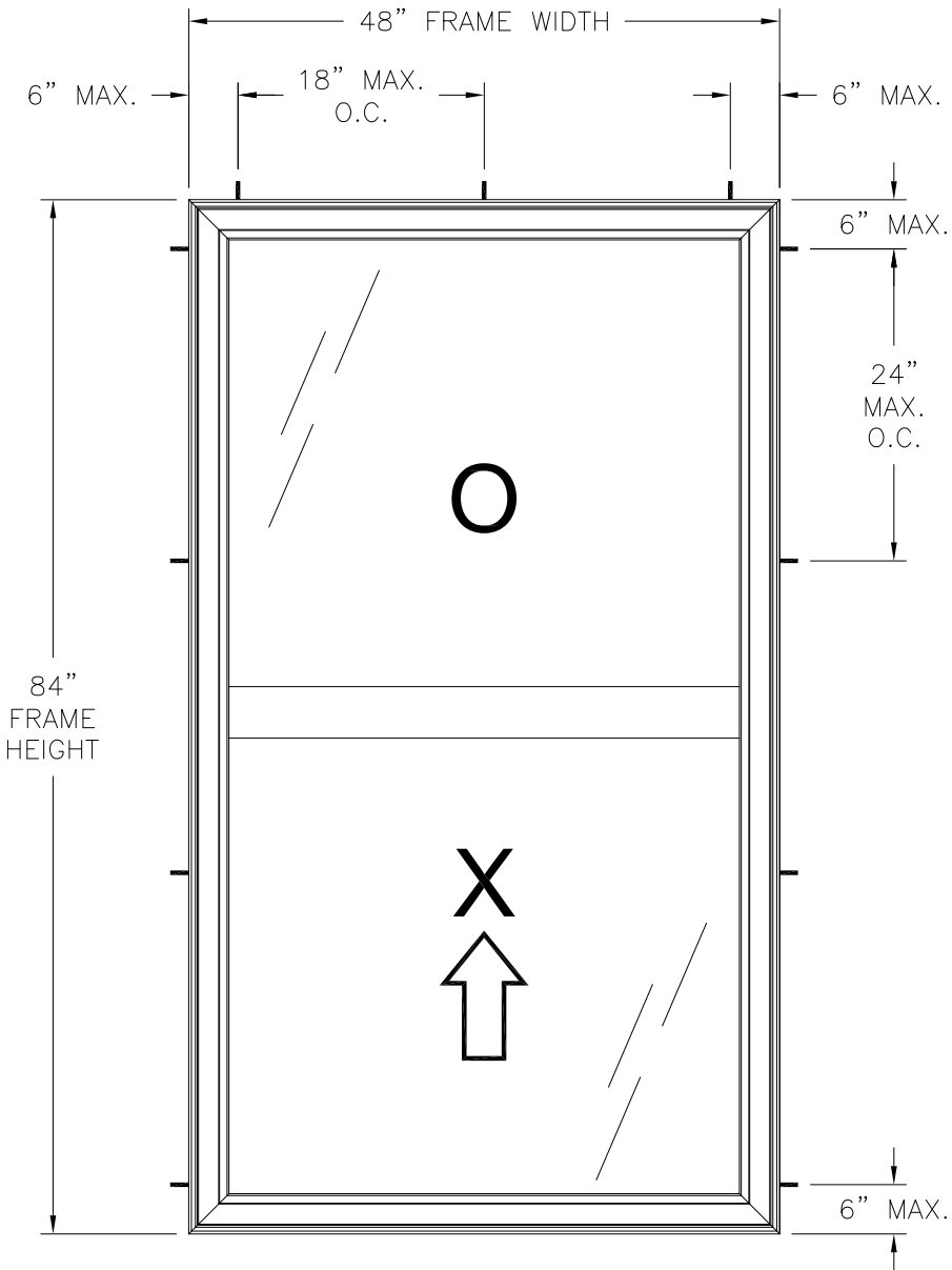
400/4000 VINYL SINGLE HUNG WINDOW EXTERIOR VIEW FRAME INSTALLATION
