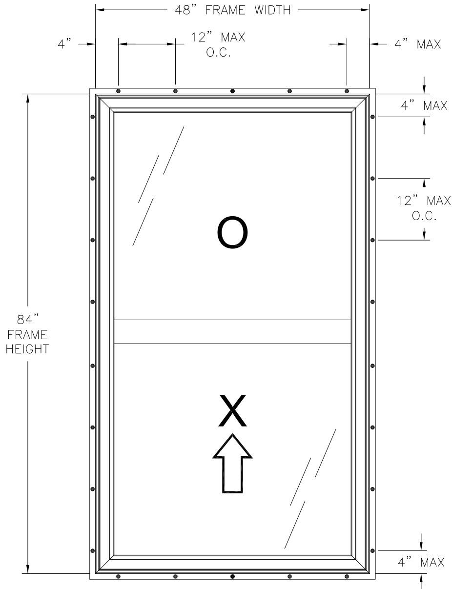
400/4000 VINYL SINGLE HUNG WINDOW EXTERIOR VIEW FIN INSTALLATION
