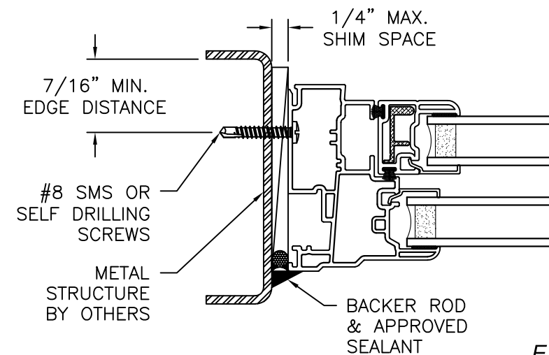
JAMB INSTALLATION DETAIL METAL STRUCTURE INSTALLATION
