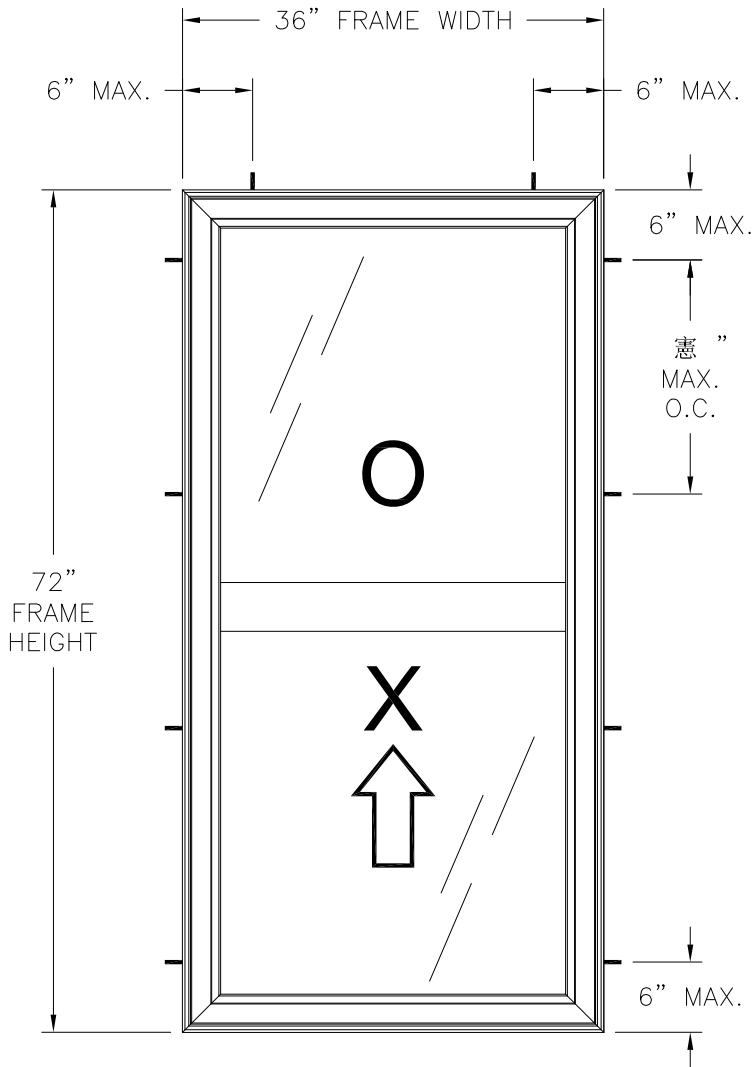
400 VINYL SINGLE HUNG WINDOW EXTERIOR VIEW FRAME INSTALLATION
