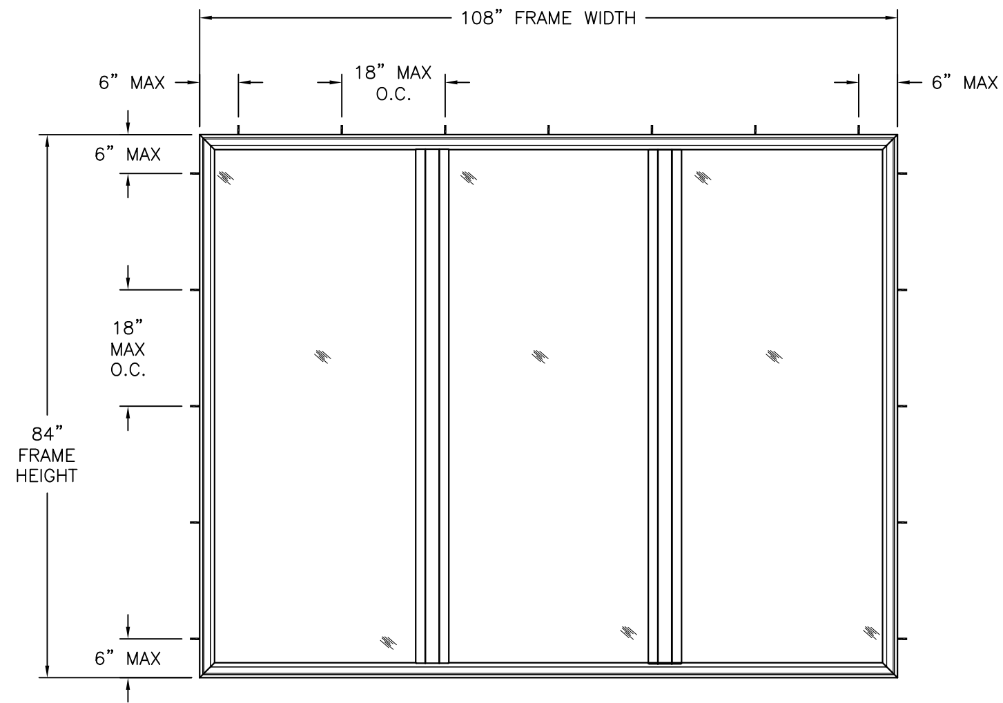
4000 VINYL TRIPLE PICTURE WINDOW EXTERIOR VIEW
