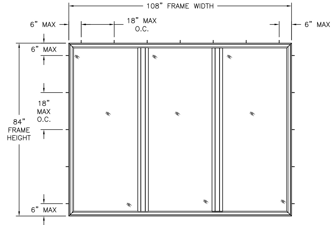
400 TRIPLE PICTURE WINDOW EXTERIOR VIEW FRAME INSTALLATION
