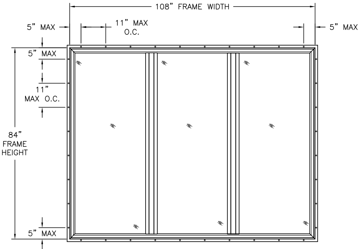
400 TRIPLE PICTURE WINDOW EXTERIOR VIEW FIN INSTALLATION
