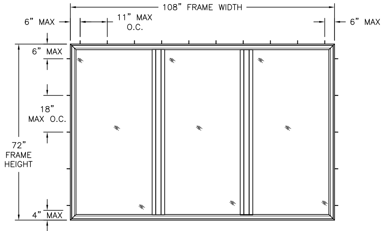
400 VINYL TRIPLE PICTURE WINDOW
