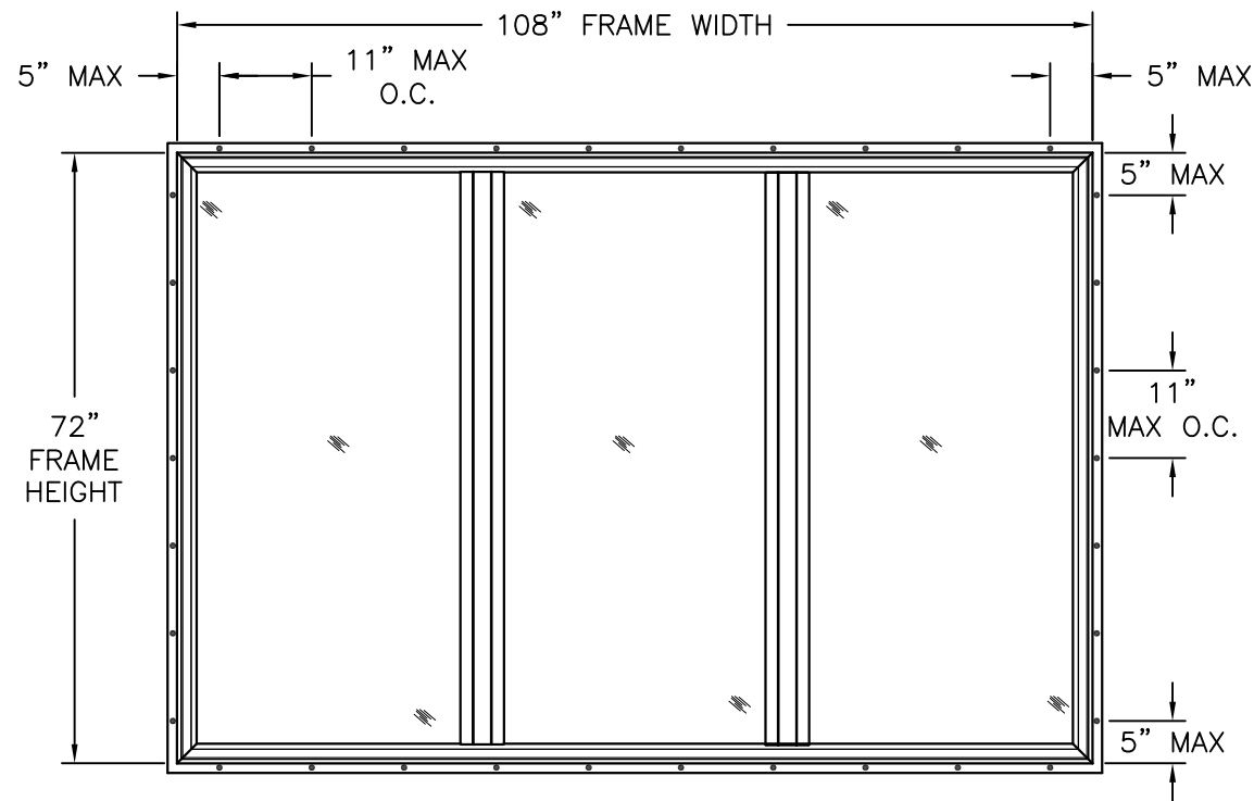
400 VINYL TRIPLE PICTURE WINDOW
