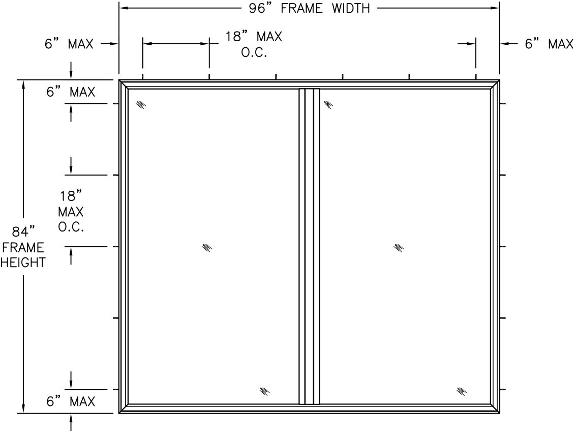
400 TWIN PICTURE WINDOW EXTERIOR VIEW FRAME INSTALLATION
