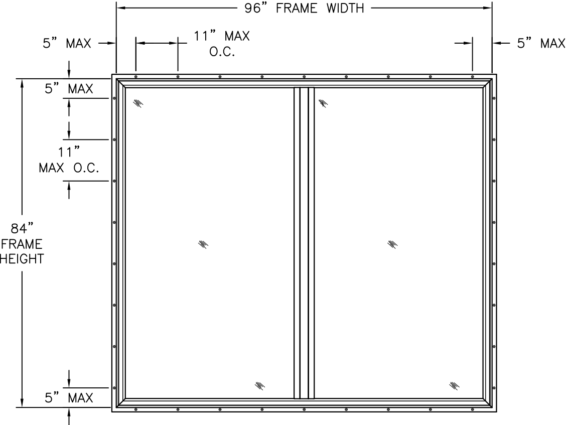
400 TWIN PICTURE WINDOW EXTERIOR VIEW FIN INSTALLATION
