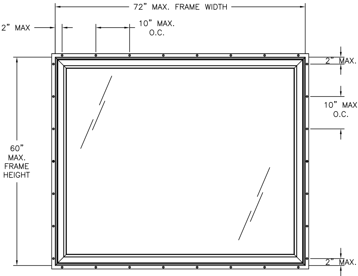
400 VINYL PICTURE WINDOW EXTERIOR VIEW FIN INSTALLATION
