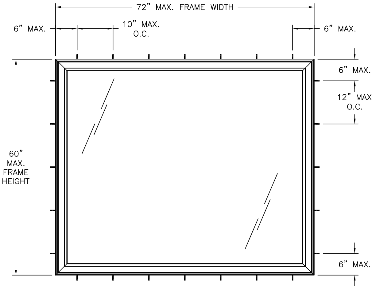
400 VINYL PICTURE WINDOW EXTERIOR VIEW FRAME INSTALLATION
