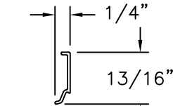
GLAZING BEAD RIGID PVC
