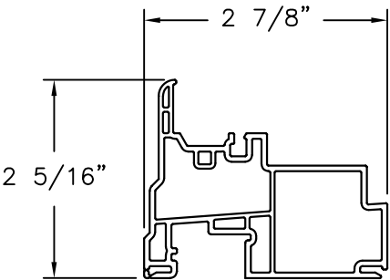
MAIN FRAME (V3823) FINLESS INSTALLATION RIGID PVC
