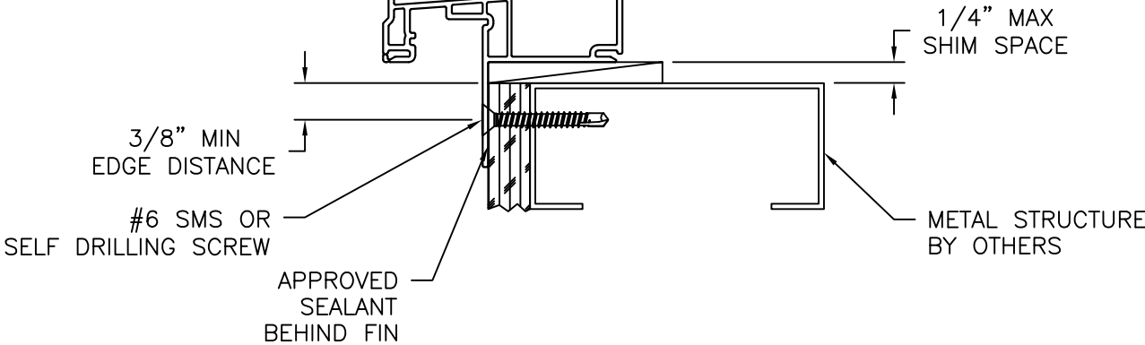
VERTICAL CROSS SECTION METAL STRUCTURE INSTALLATION
