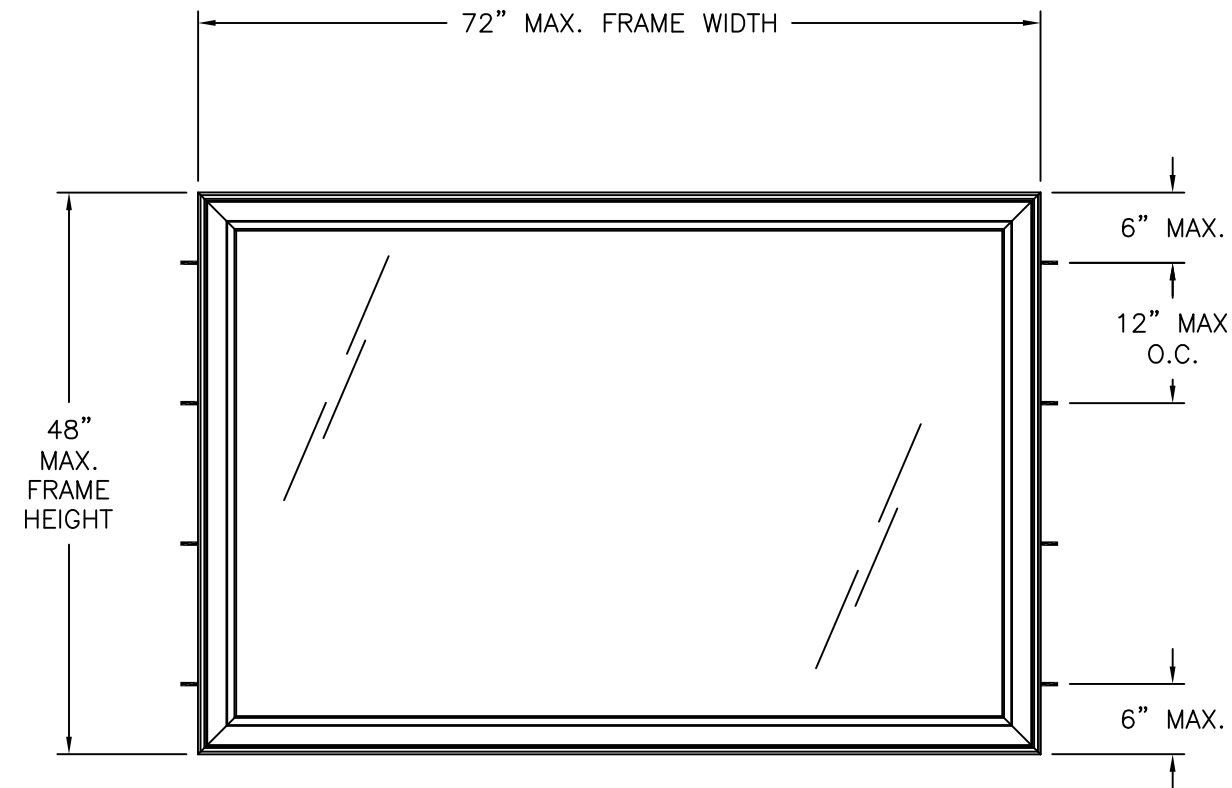
400 VINYL PICTURE WINDOW EXTERIOR VIEW FRAME INSTALLATION
