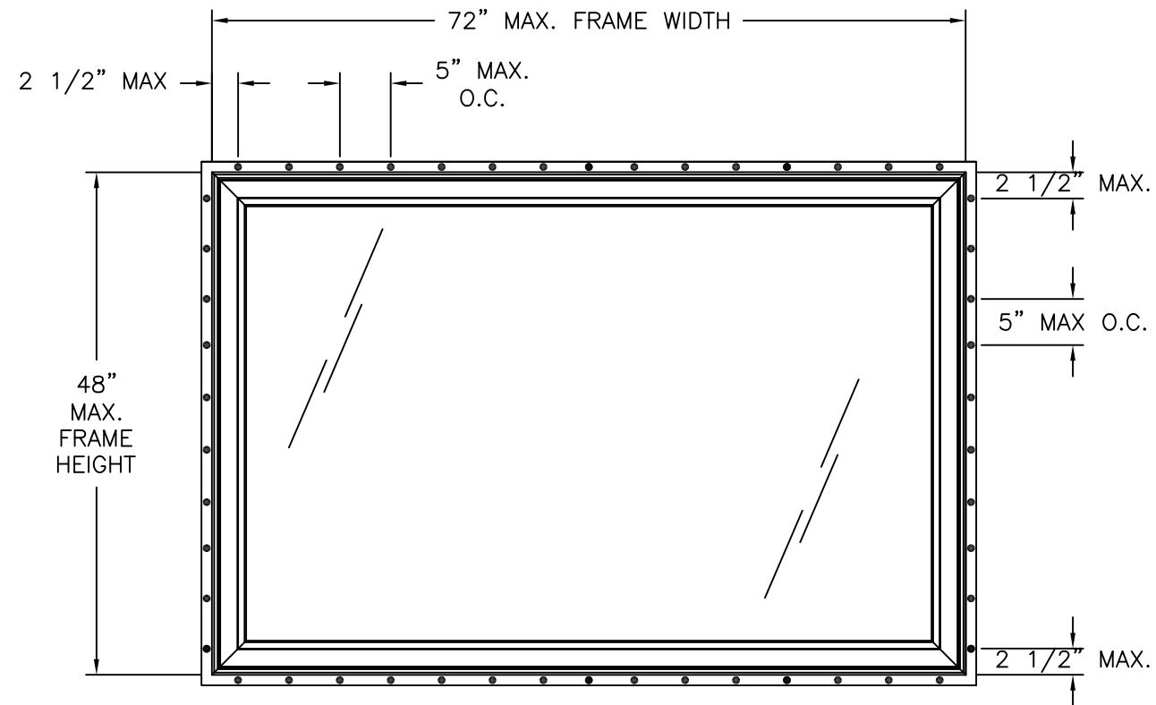
400 VINYL PICTURE WINDOW EXTERIOR VIEW FIN INSTALLATION
