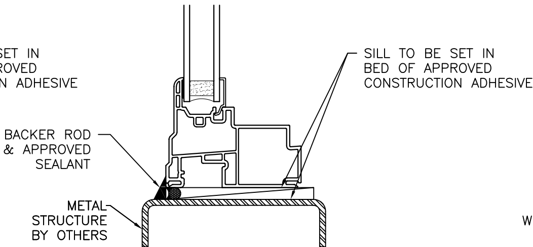
EXTERIOR
