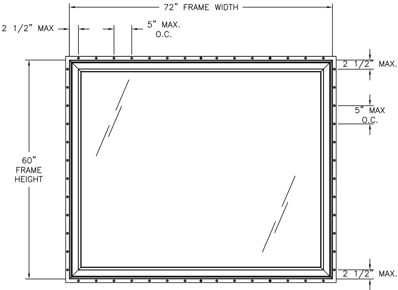
400 VINYL PICTURE WINDOW EXTERIOR VIEW FIN INSTALLATION
