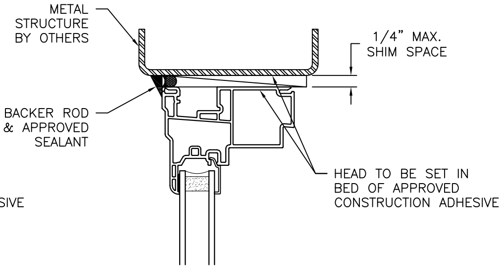
EXTERIOR
