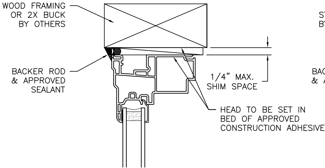
EXTERIOR
