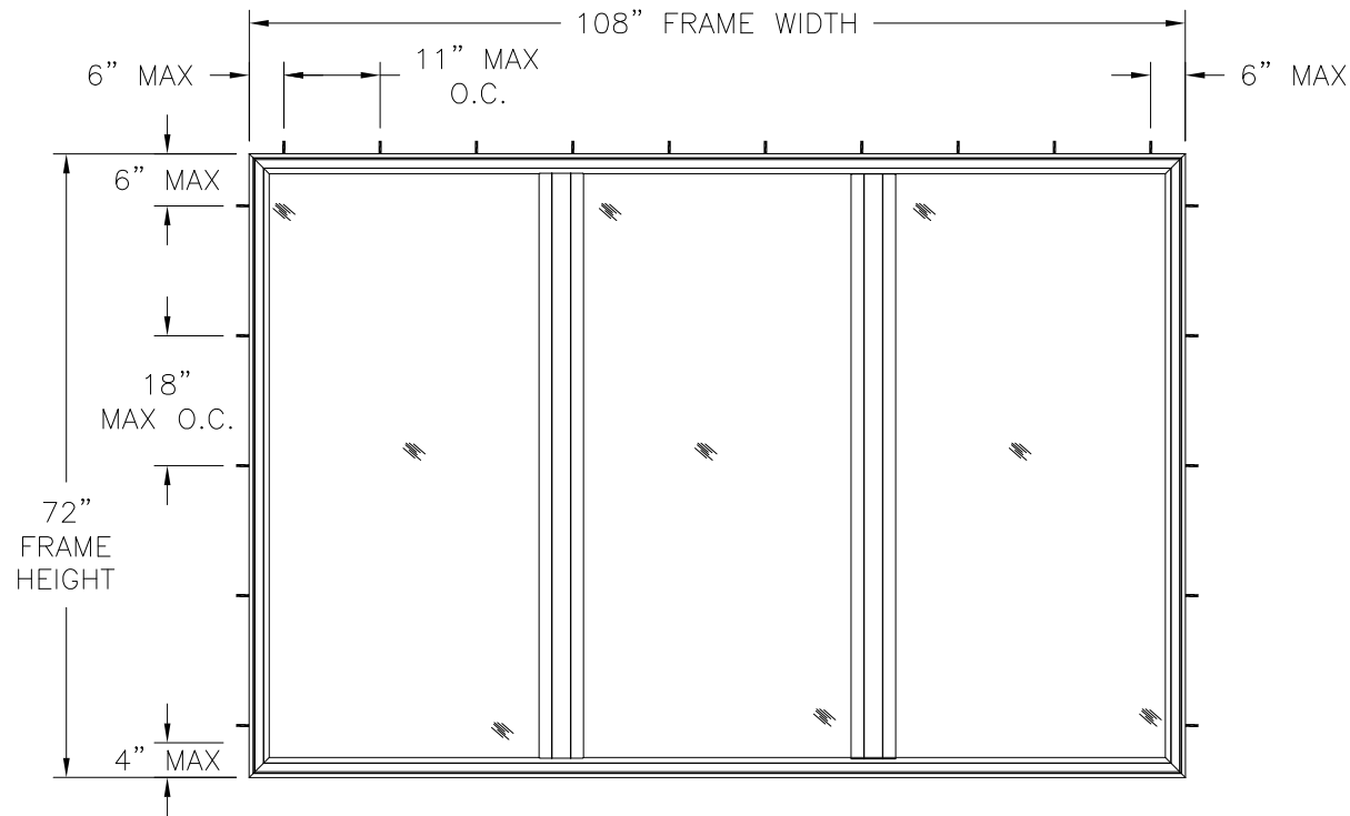
400 VINYL TRIPLE PICTURE WINDOW EXTERIOR VIEW FRAME INSTALLATION
