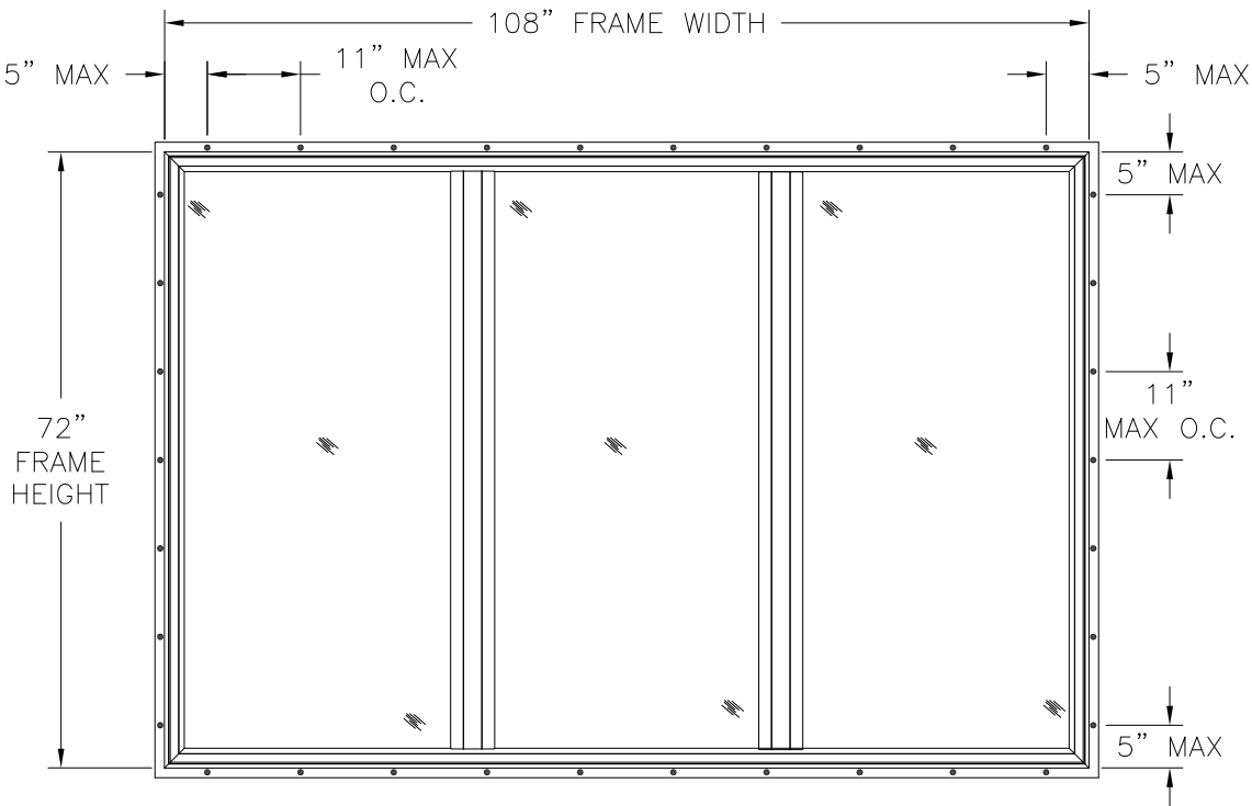
400 VINYL TRIPLE PICTURE WINDOW EXTERIOR VIEW FIN INSTALLATION
