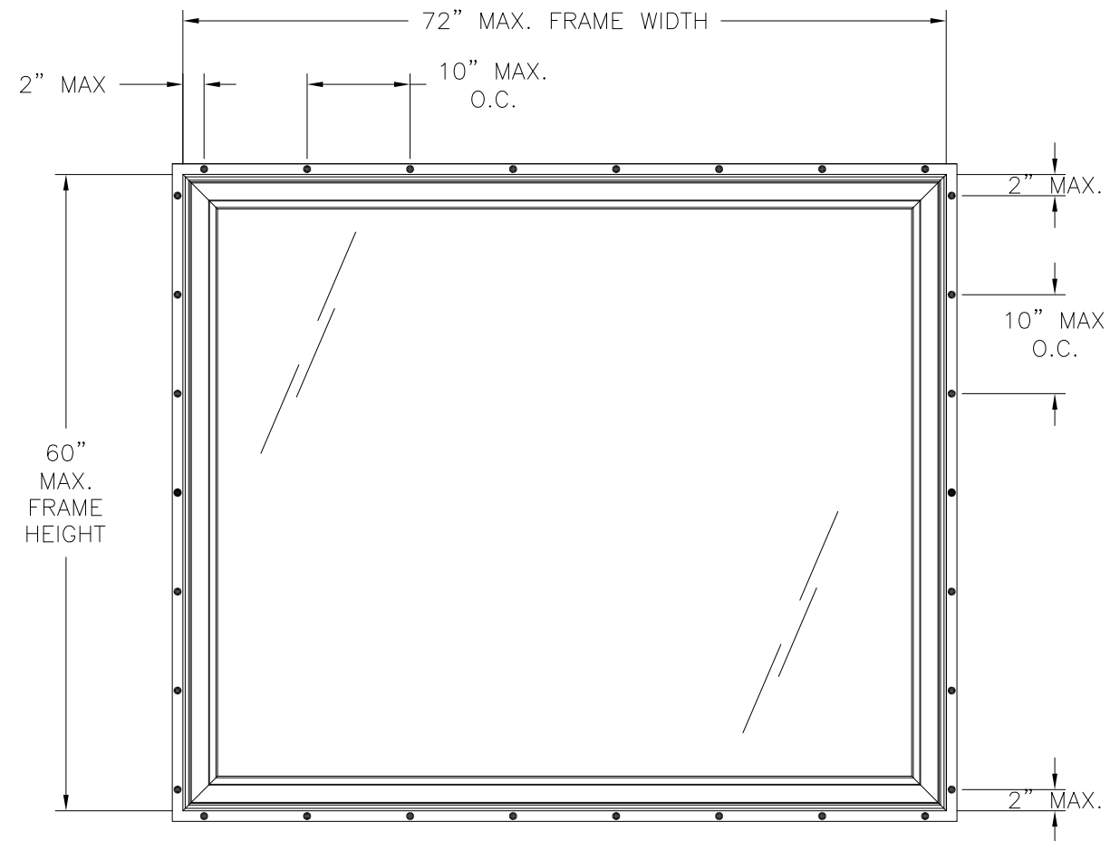
400 VINYL PICTURE WINDOW EXTERIOR VIEW FIN INSTALLATION
